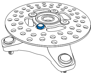
Magnetic Bolt Installation ATV Rotor
