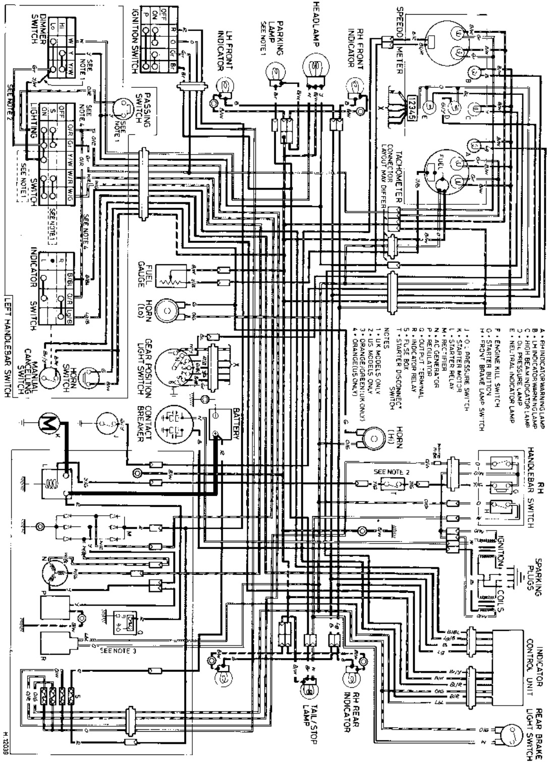
Wiring diagram GS1000 L model
