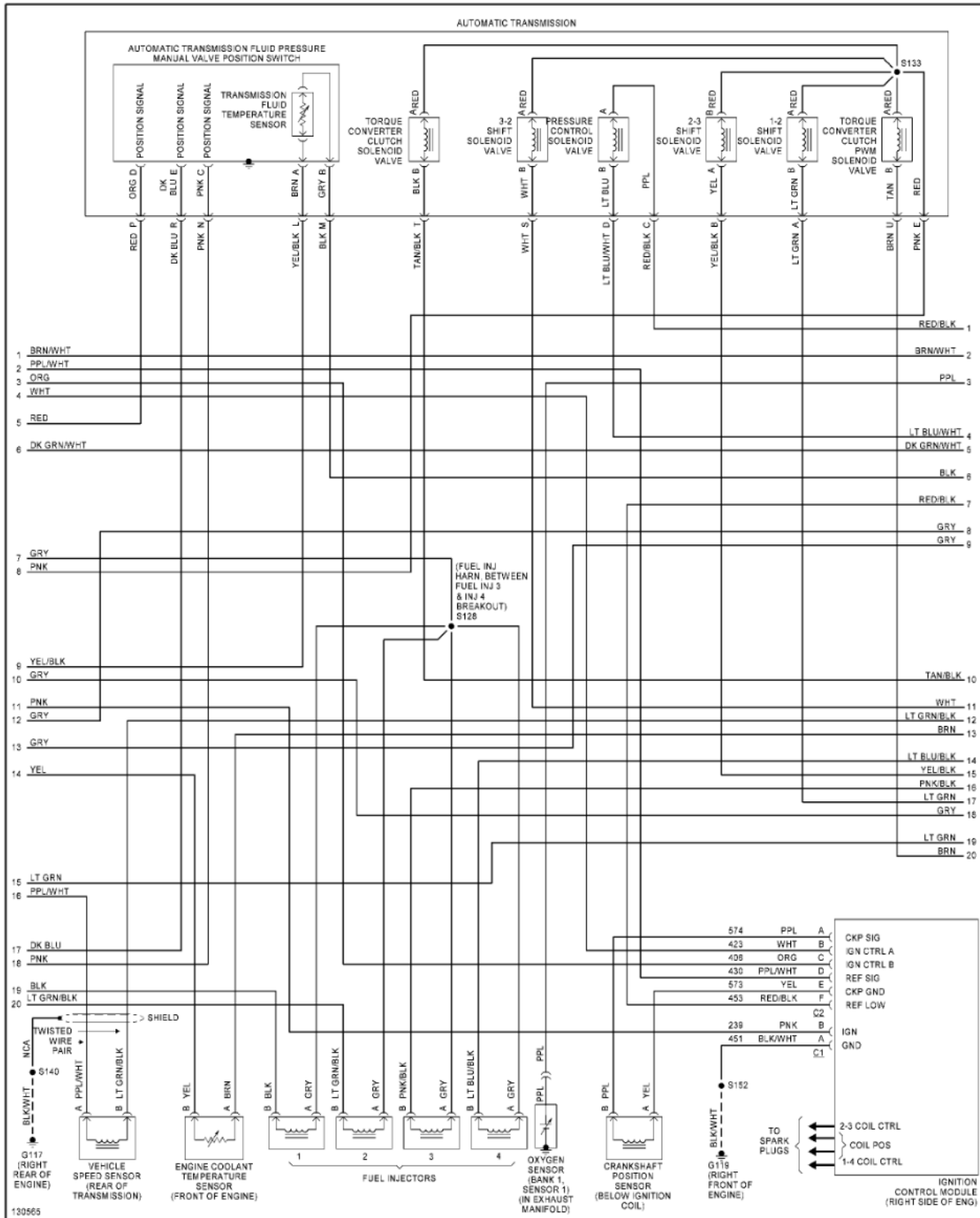
Fig. 18: 2.2L VIN 4, Engine Performance Circuits (2 of 3)
