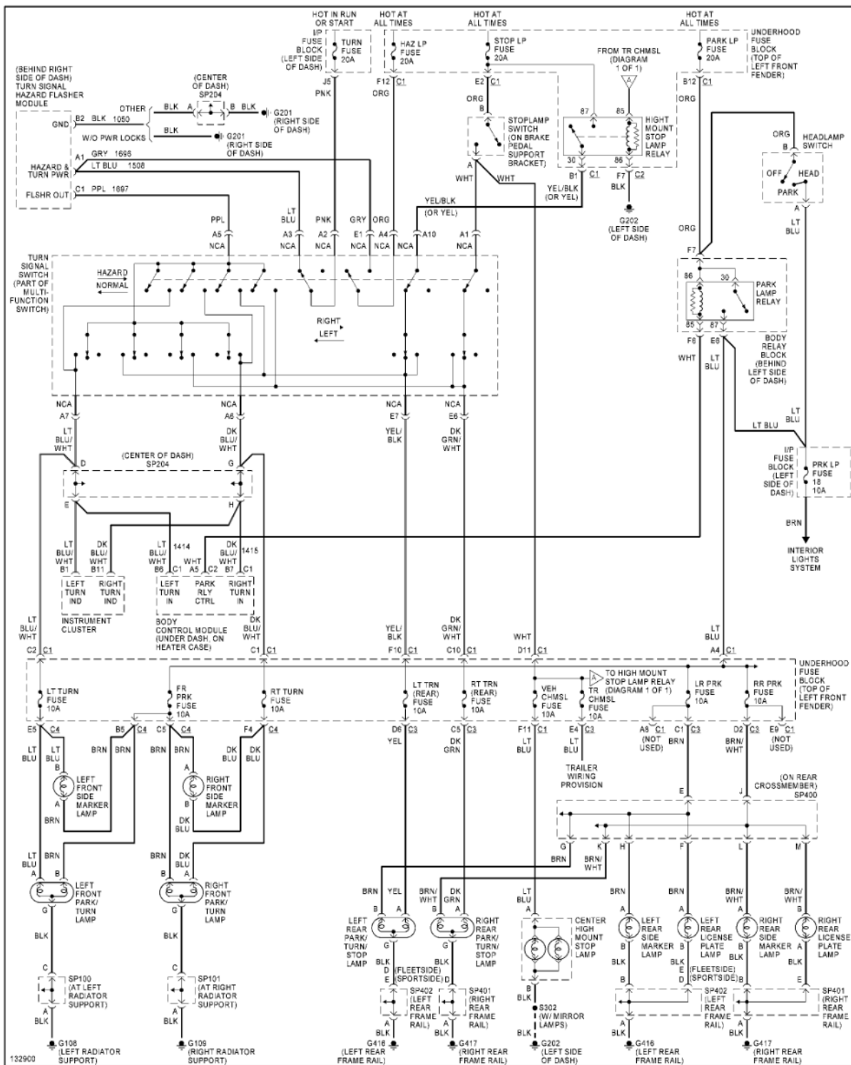
Fig. 28: Exterior Lamps Circuit
