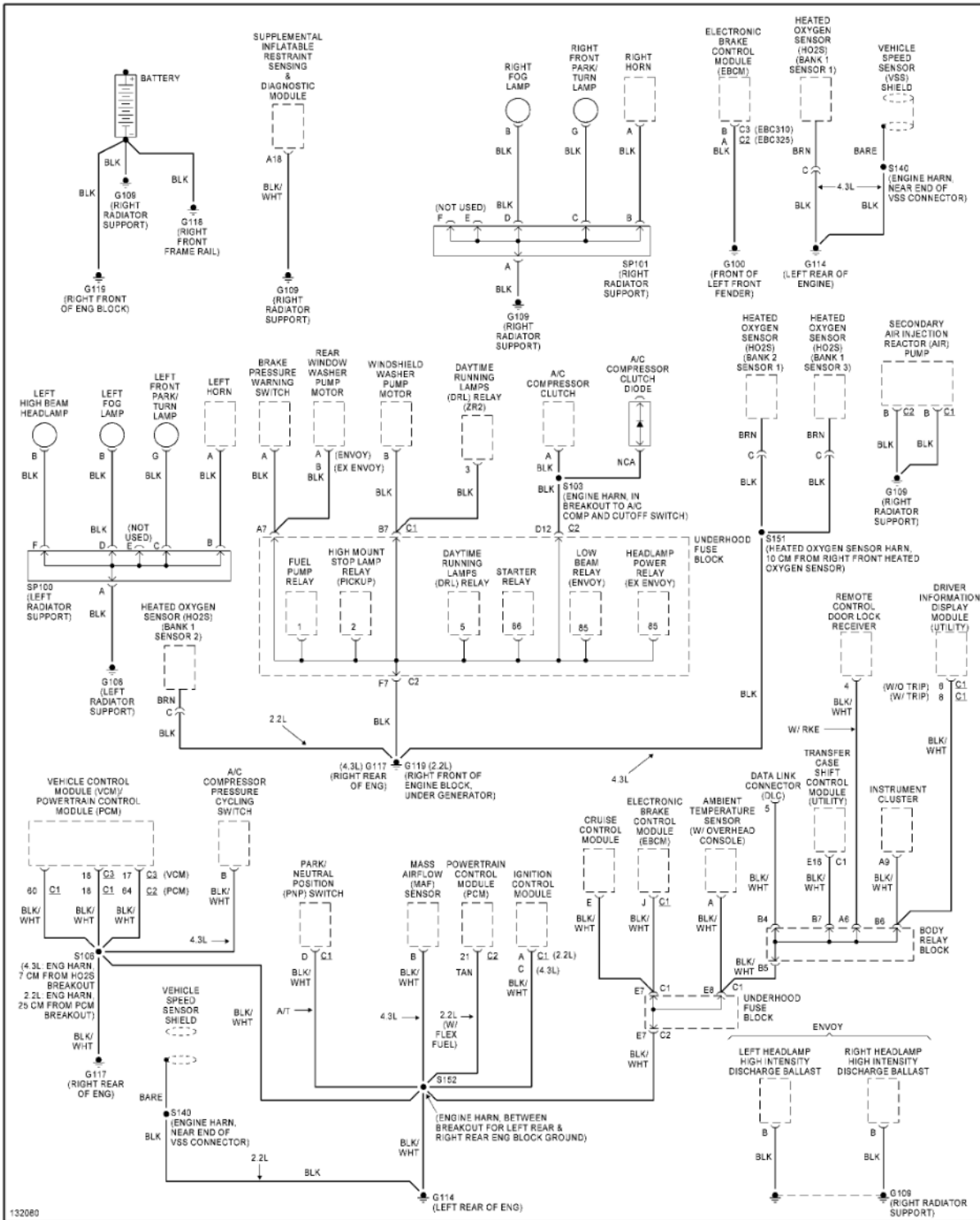
Fig. 29: Ground Distribution Circuit (1 of 3)
