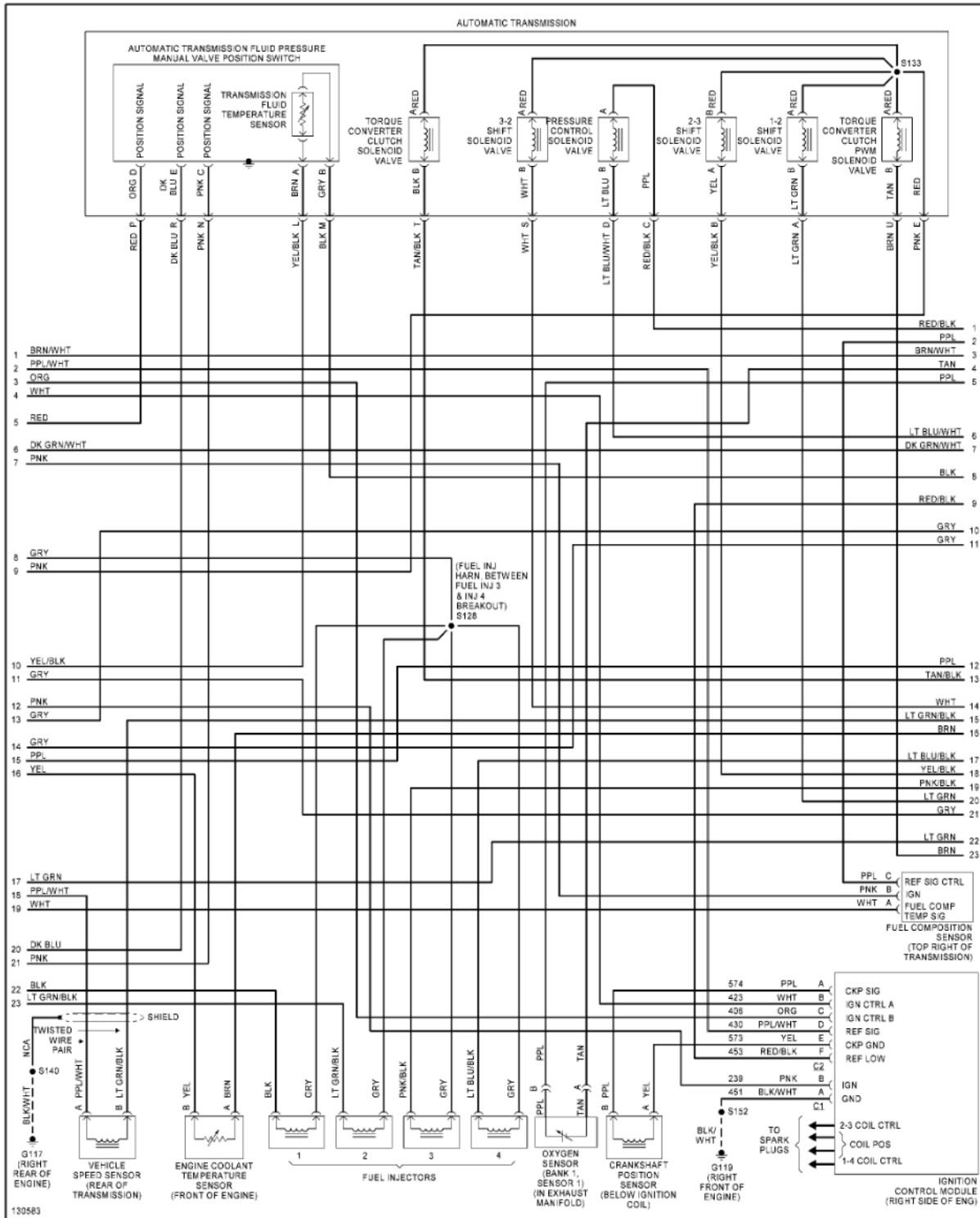
Fig. 21: 2.2L VIN 5, Engine Performance Circuits (2 of 3)
