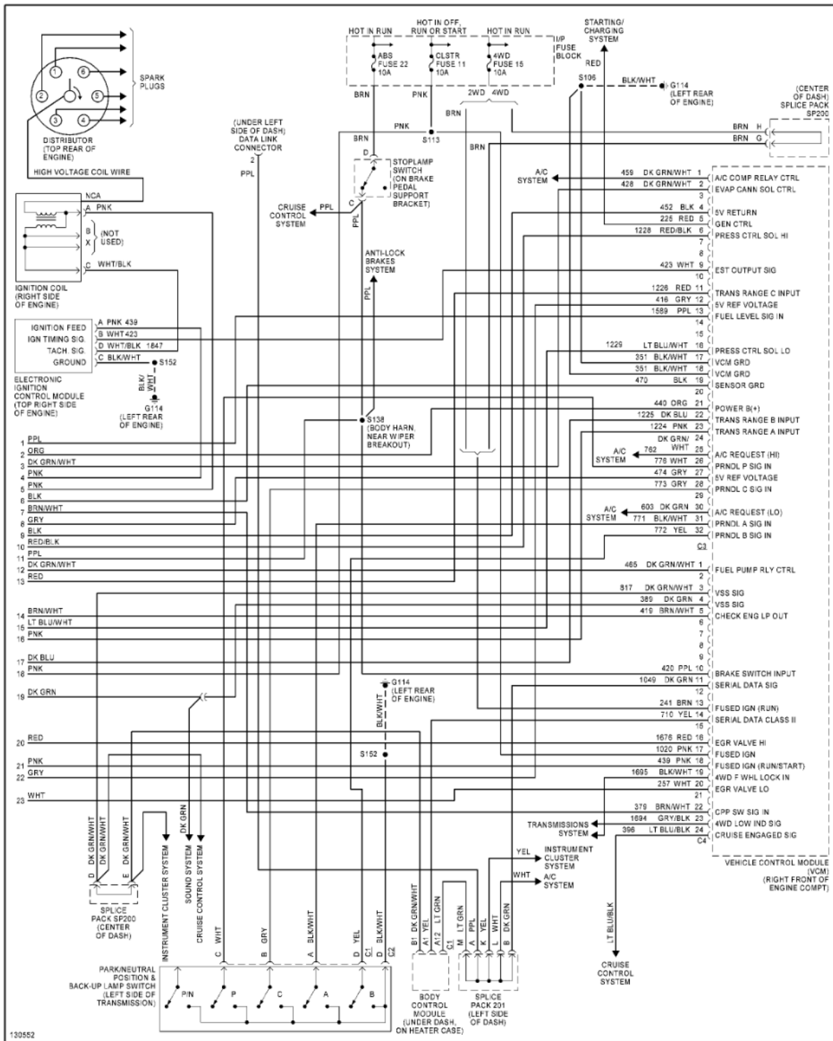
Fig. 26: 4.3L VIN W, Engine Performance Circuits (4 of 4)
