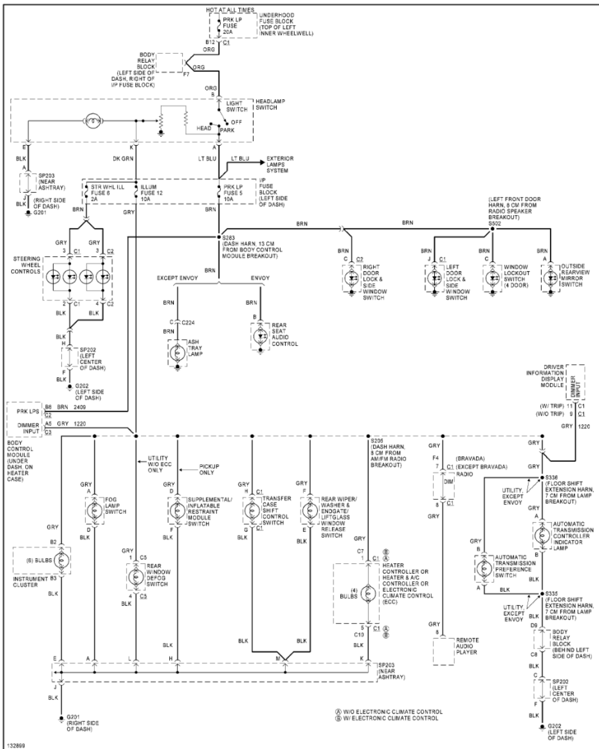
Fig. 38: Instrument Illumination Circuit
