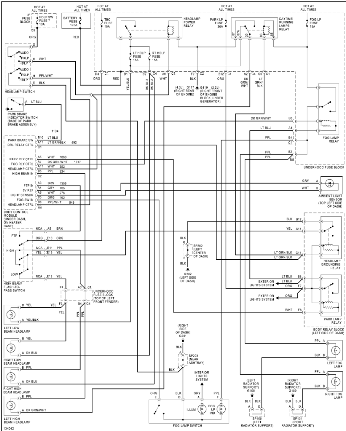
Fig. 33: Headlight Circuit, W/O ZR2
