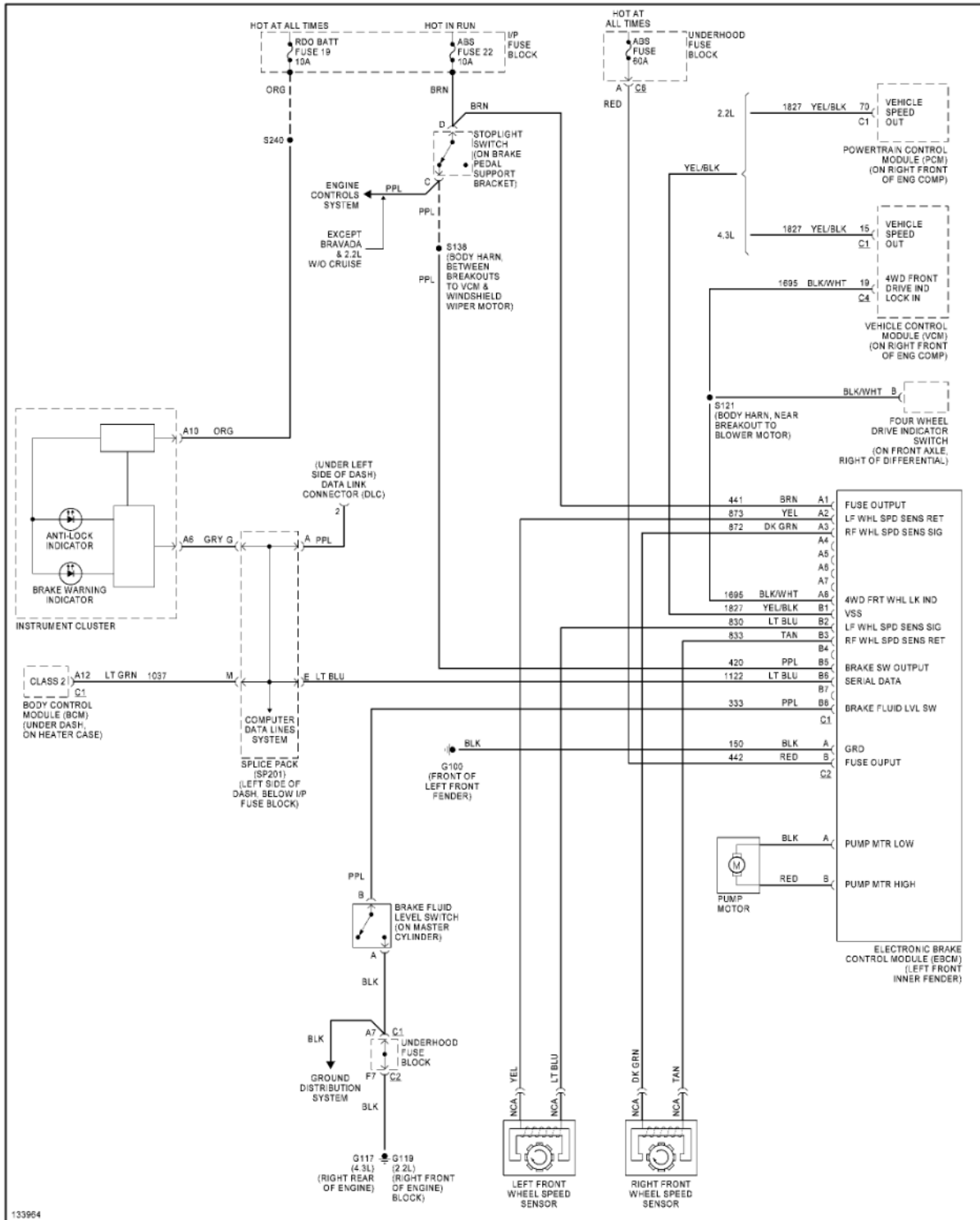
Fig. 10: Anti-lock Brake Circuits, 325 ABS
