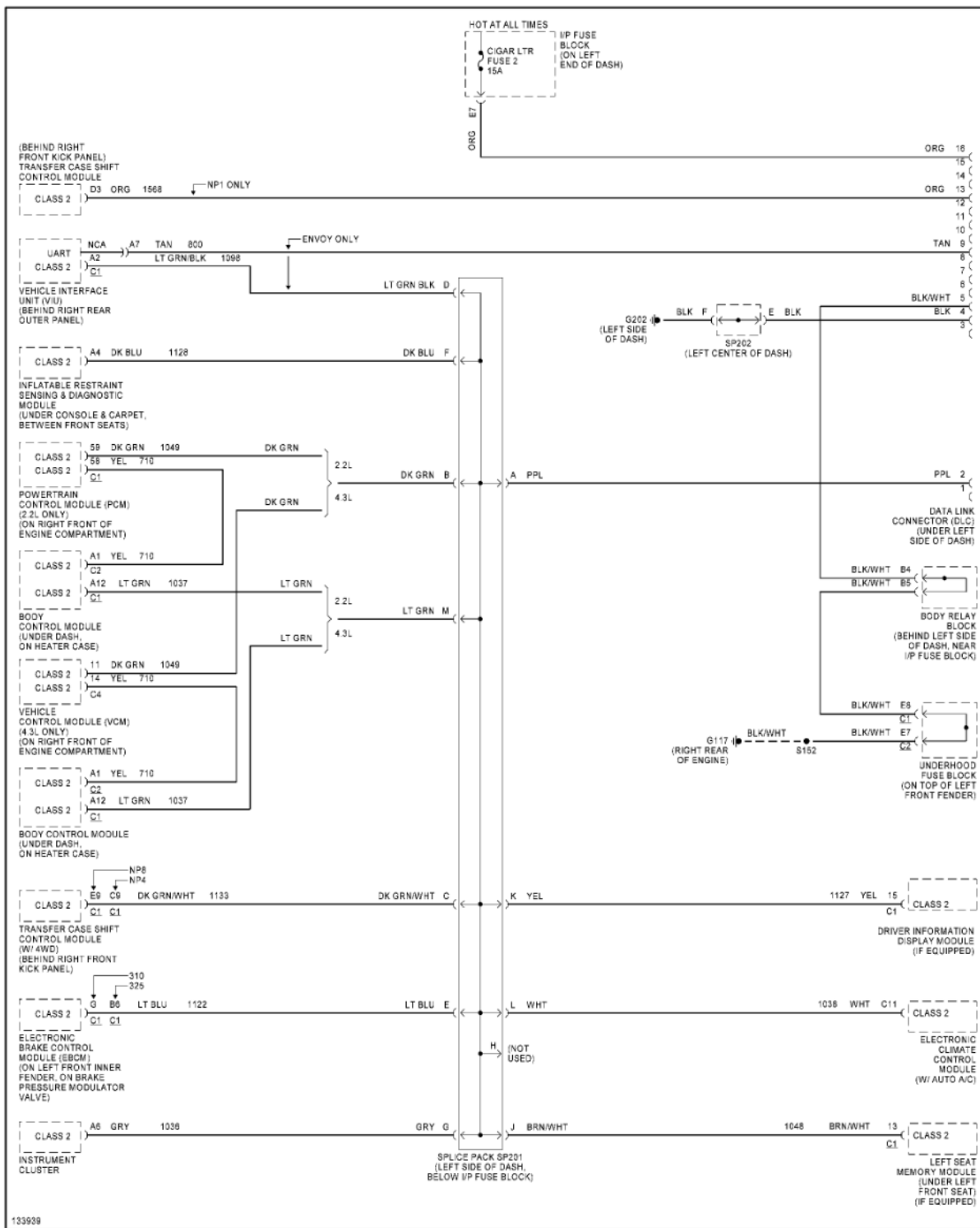
Fig. 14: Computer Data Lines
