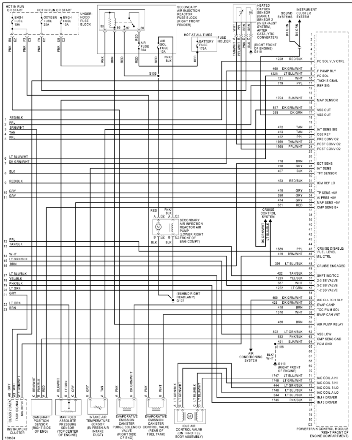
Fig. 22: 2.2L VIN 5, Engine Performance Circuits (3 of 3)
