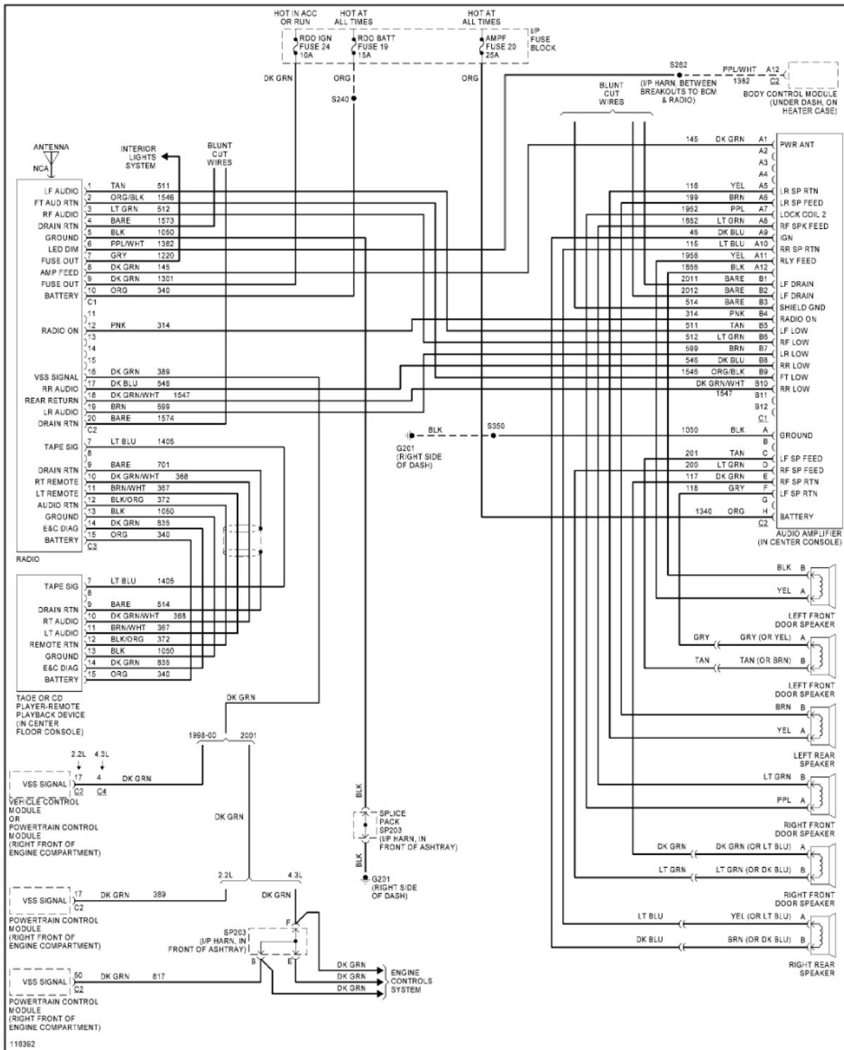
Fig. 52: Radio Circuits, W/ Amplifier
