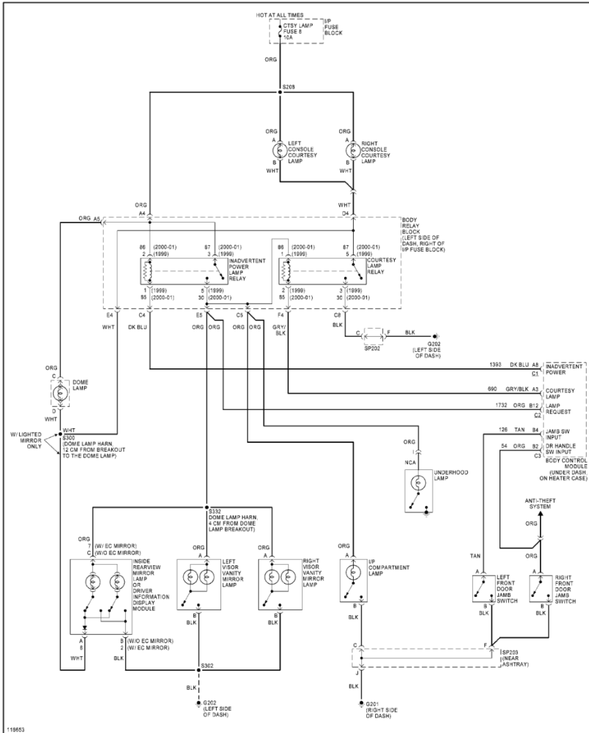
Fig. 37: Courtesy Lamps Circuit
