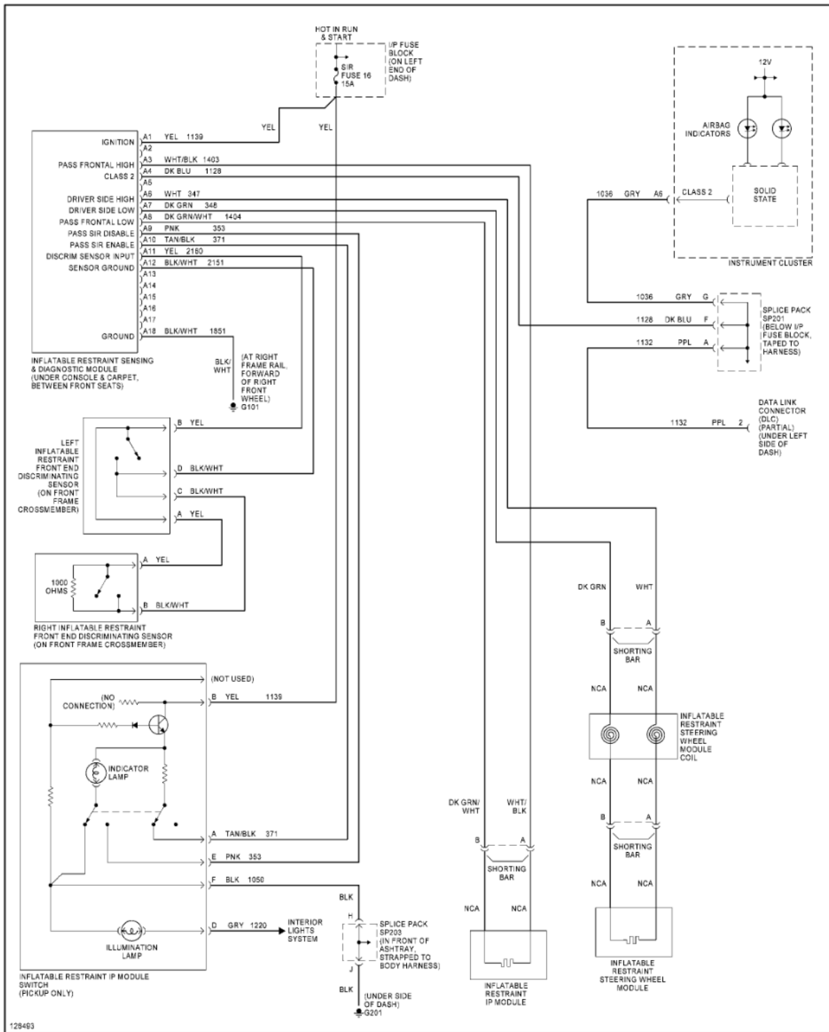
Fig. 57: Supplemental Restraint Circuit
