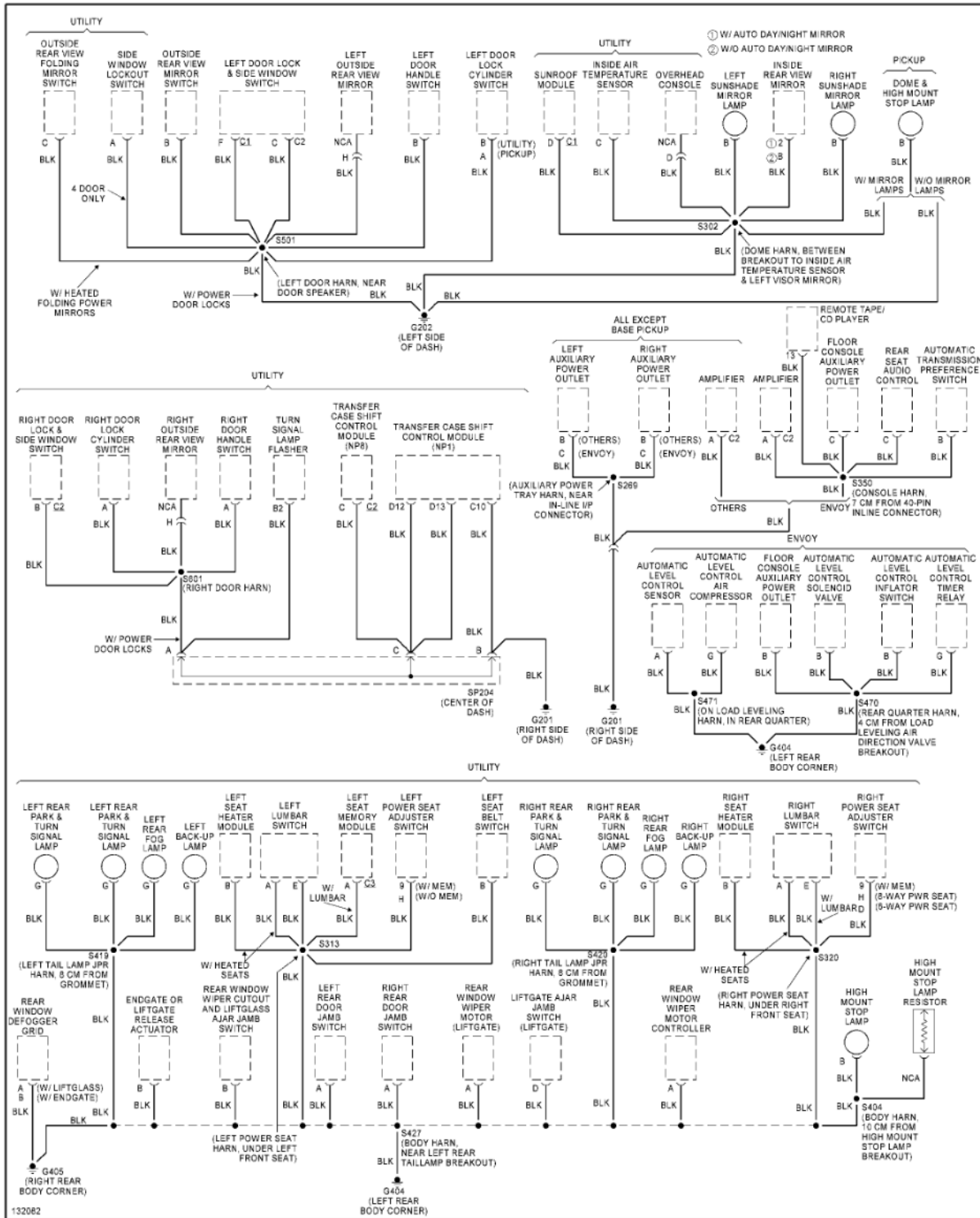
Fig. 31: Ground Distribution Circuit (3 of 3)
