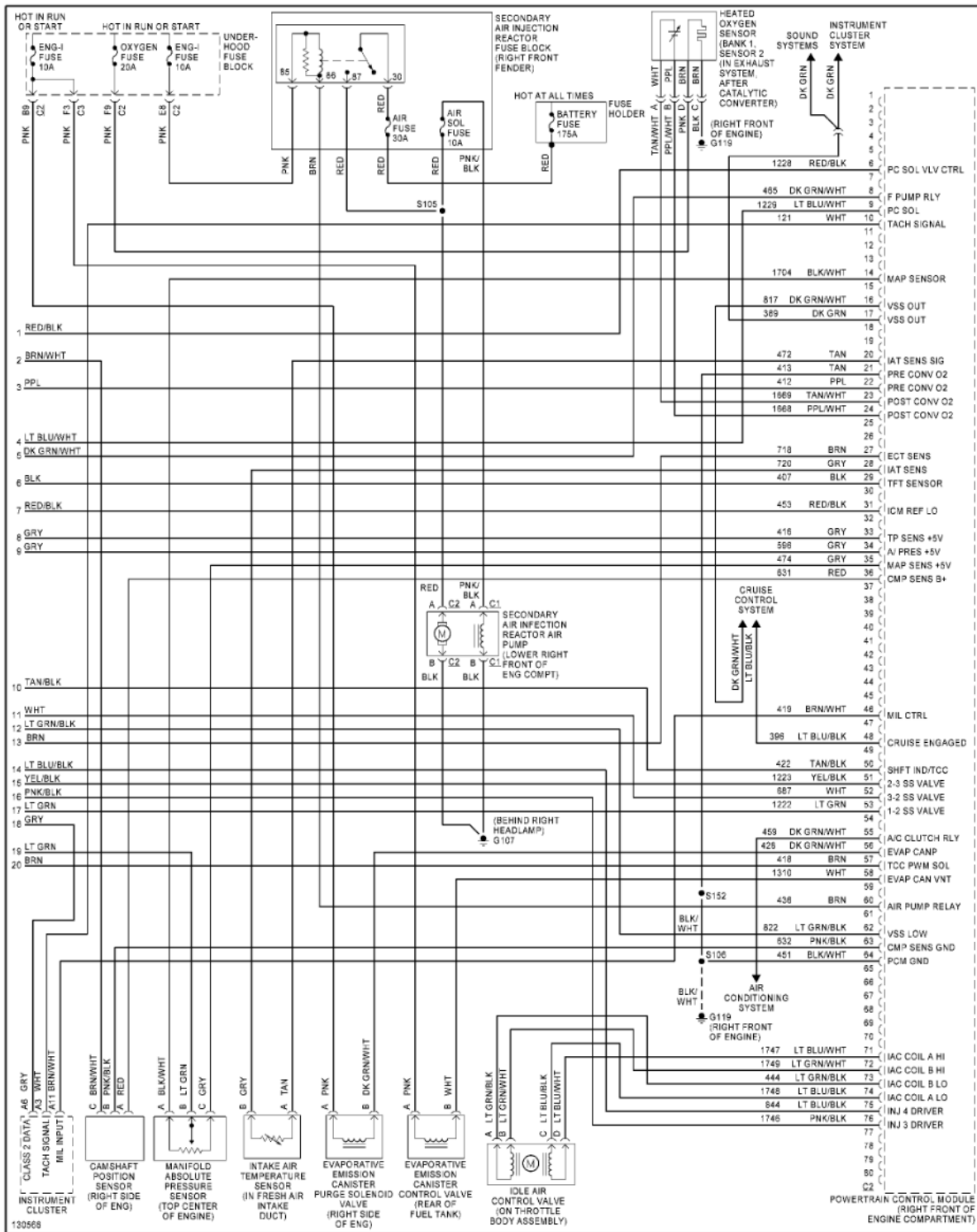
Fig. 19: 2.2L VIN 4, Engine Performance Circuits (3 of 3)
