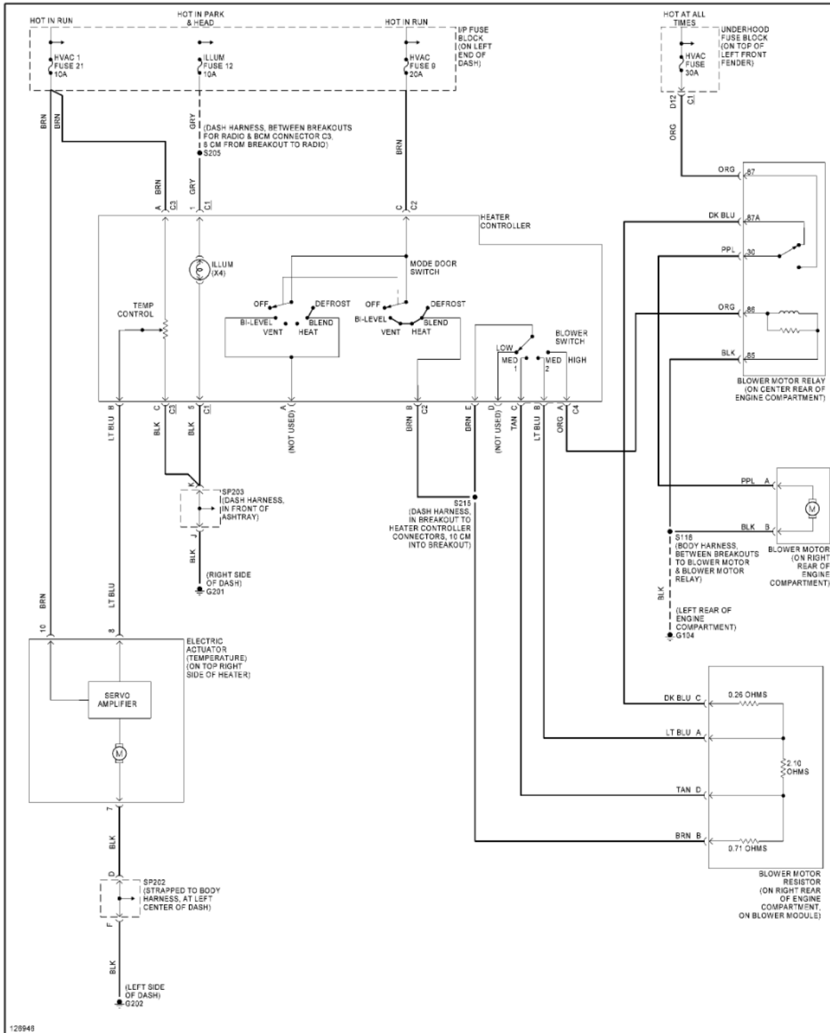
Fig. 3: Heater Circuit
