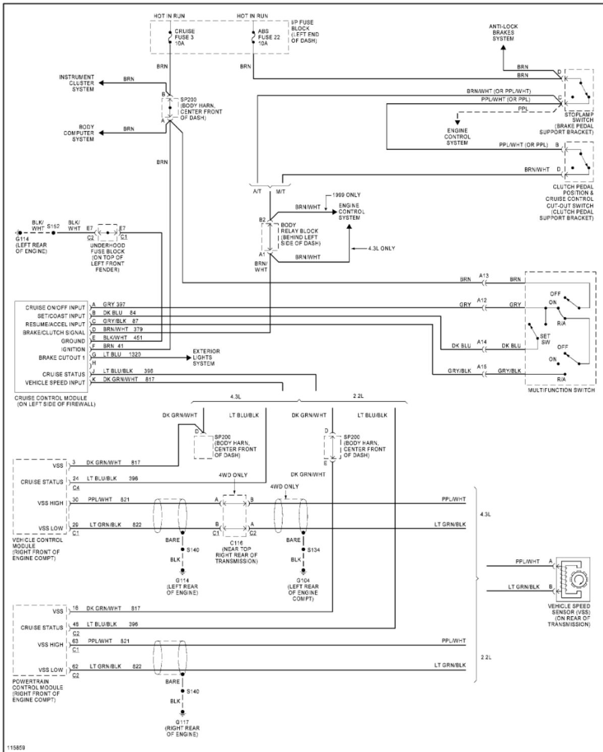
Fig. 15: Cruise Control Circuit
