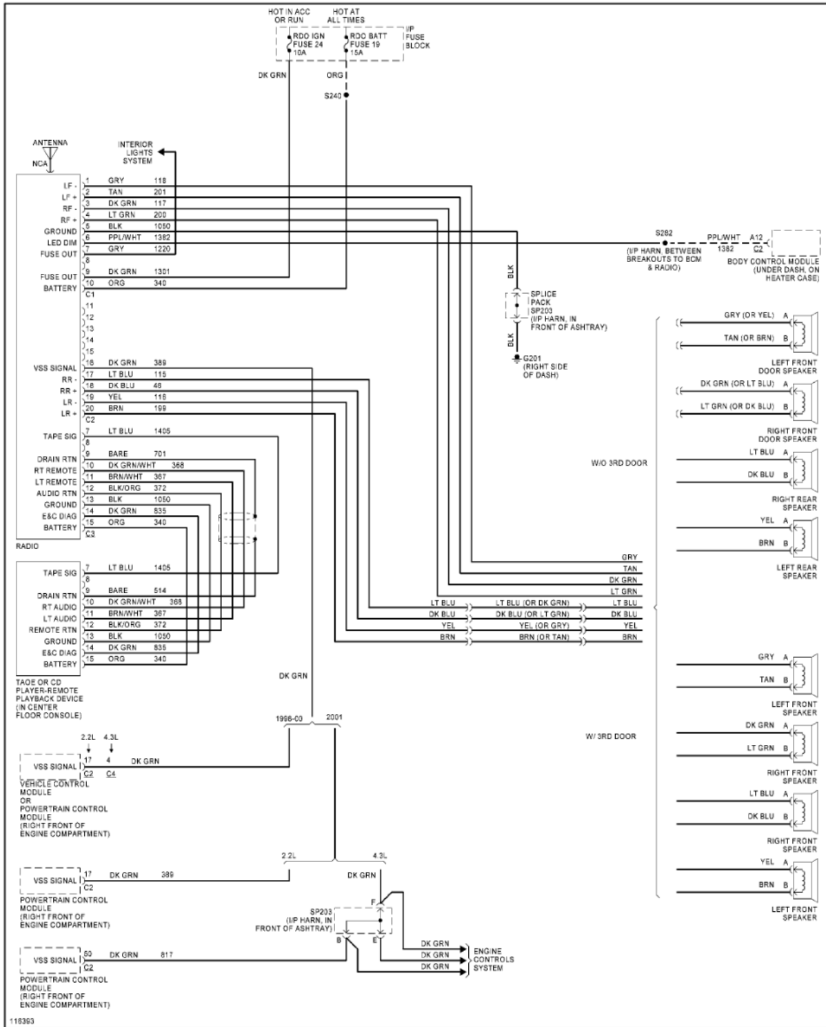
Fig. 53: Radio Circuits, W/O Amplifier
