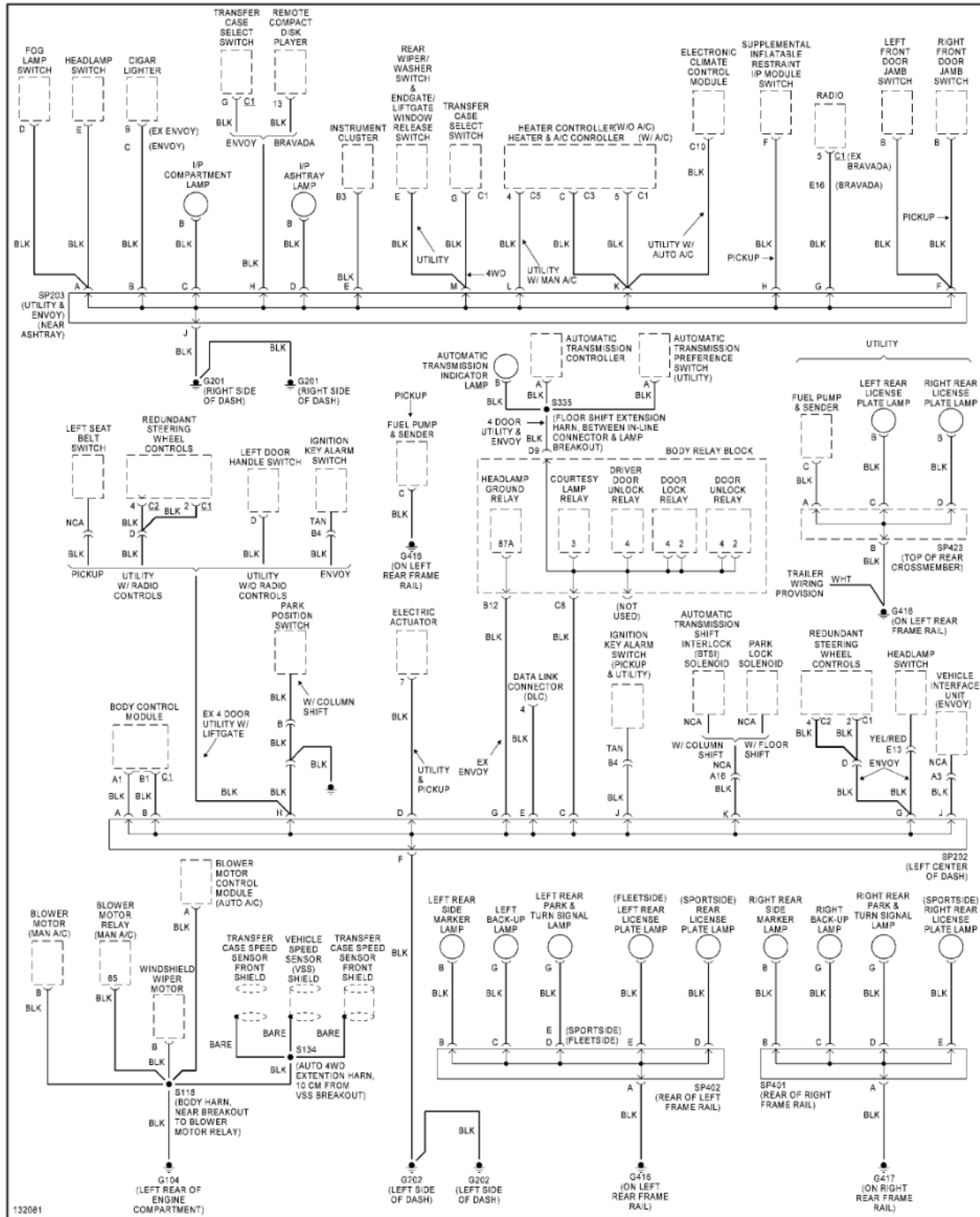
Fig. 30: Ground Distribution Circuit (2 of 3)
