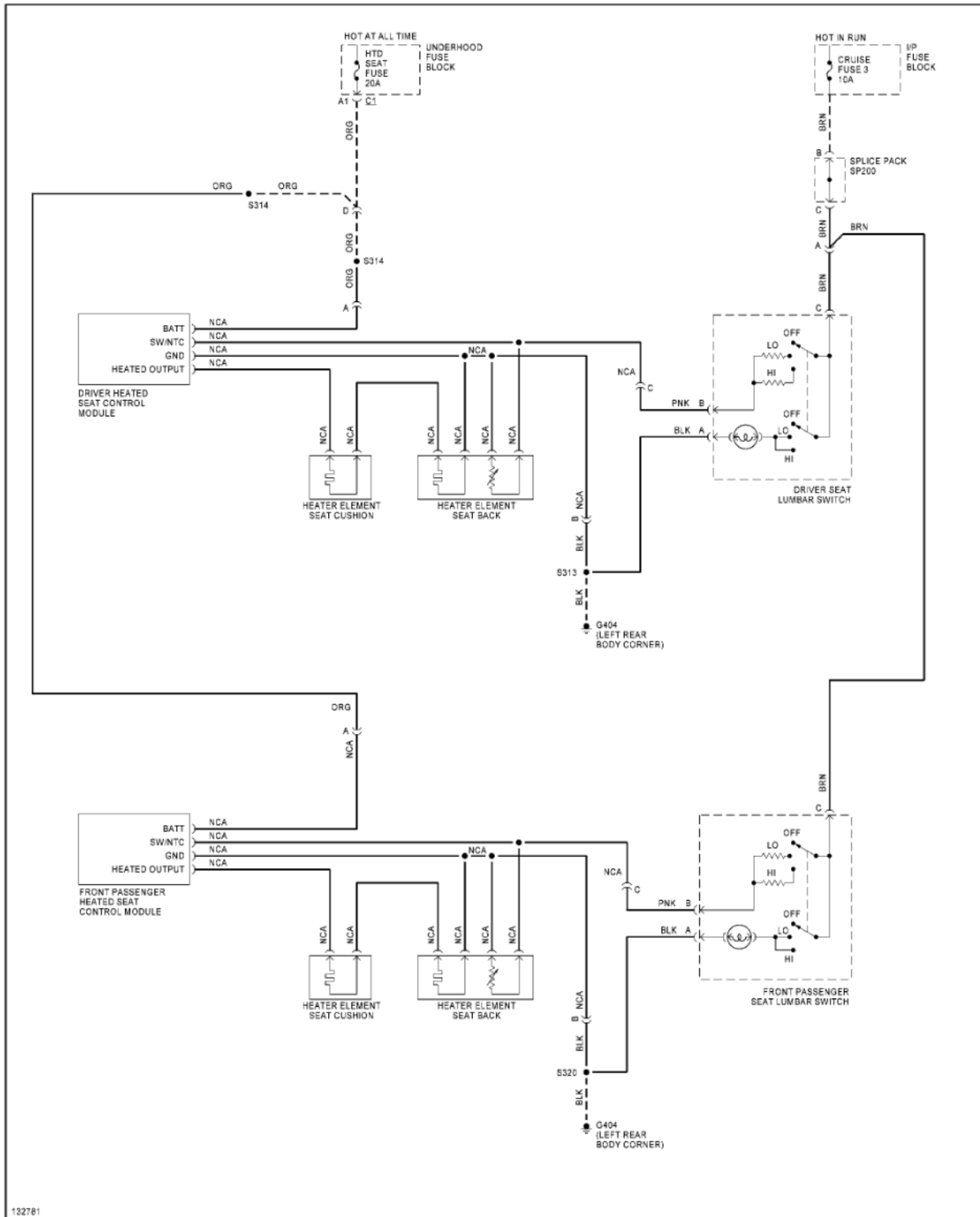
Fig. 49: Heated Seats Circuit
