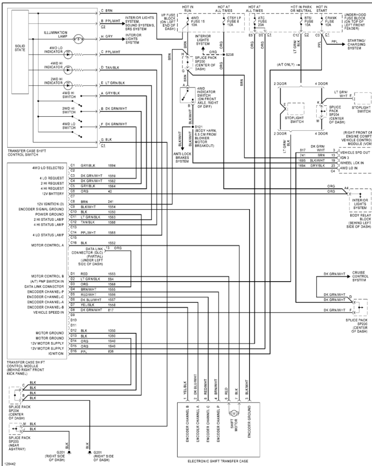
Fig. 60: 4WD Circuit, W/ 2-Speed Selectable Transfer Case
