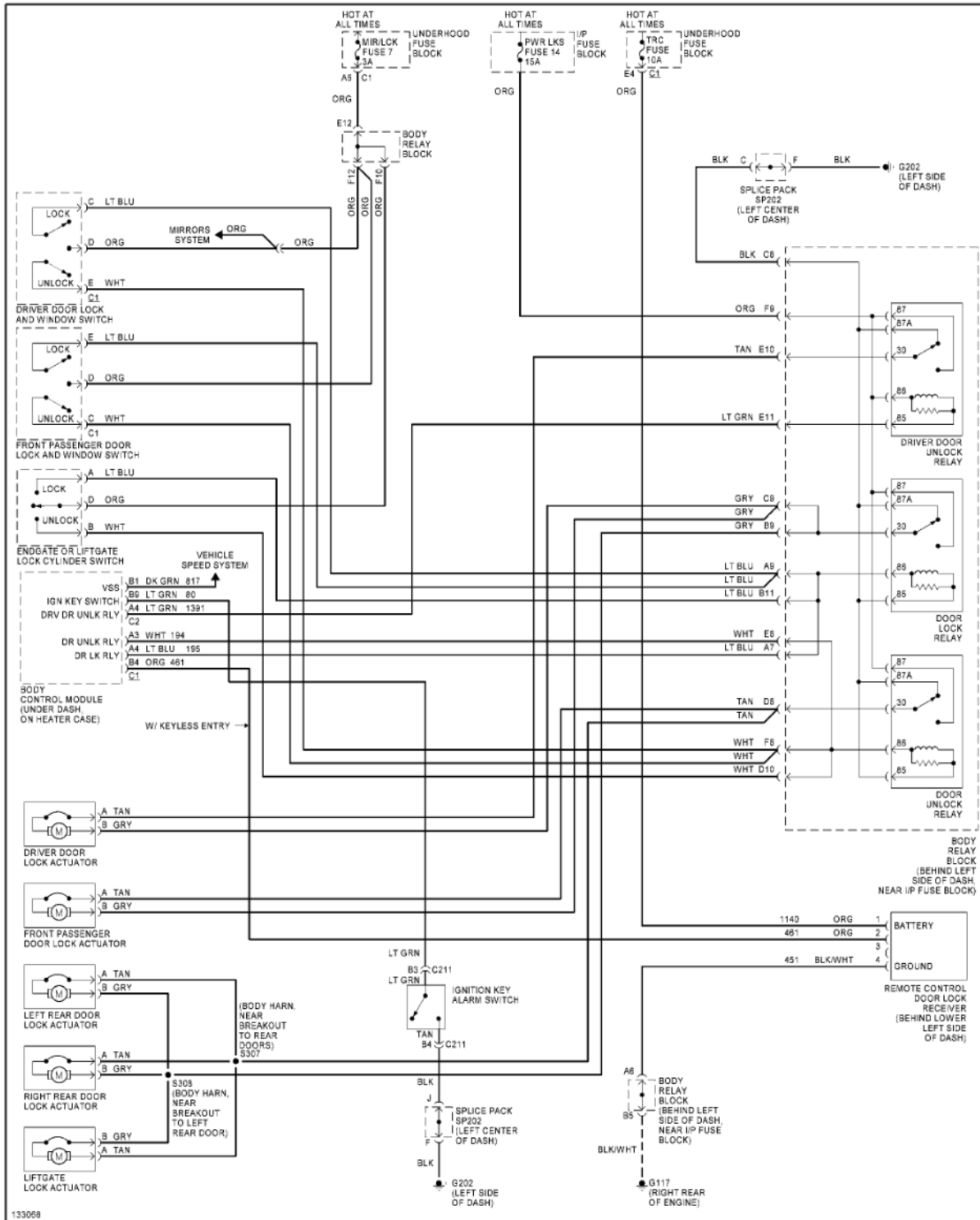
Fig. 44: Power Door Lock Circuit
