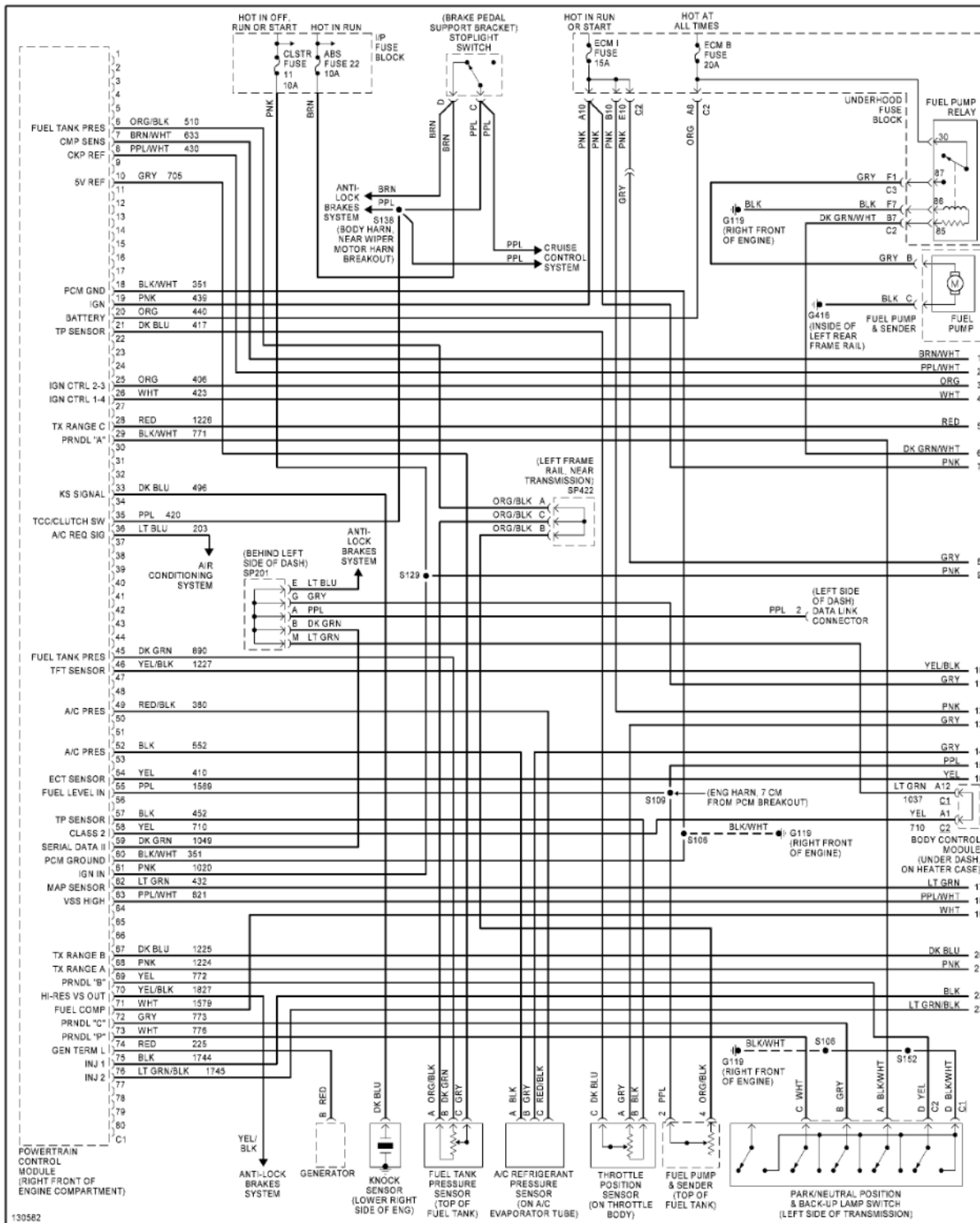
Fig. 20: 2.2L VIN 5, Engine Performance Circuits (1 of 3)
