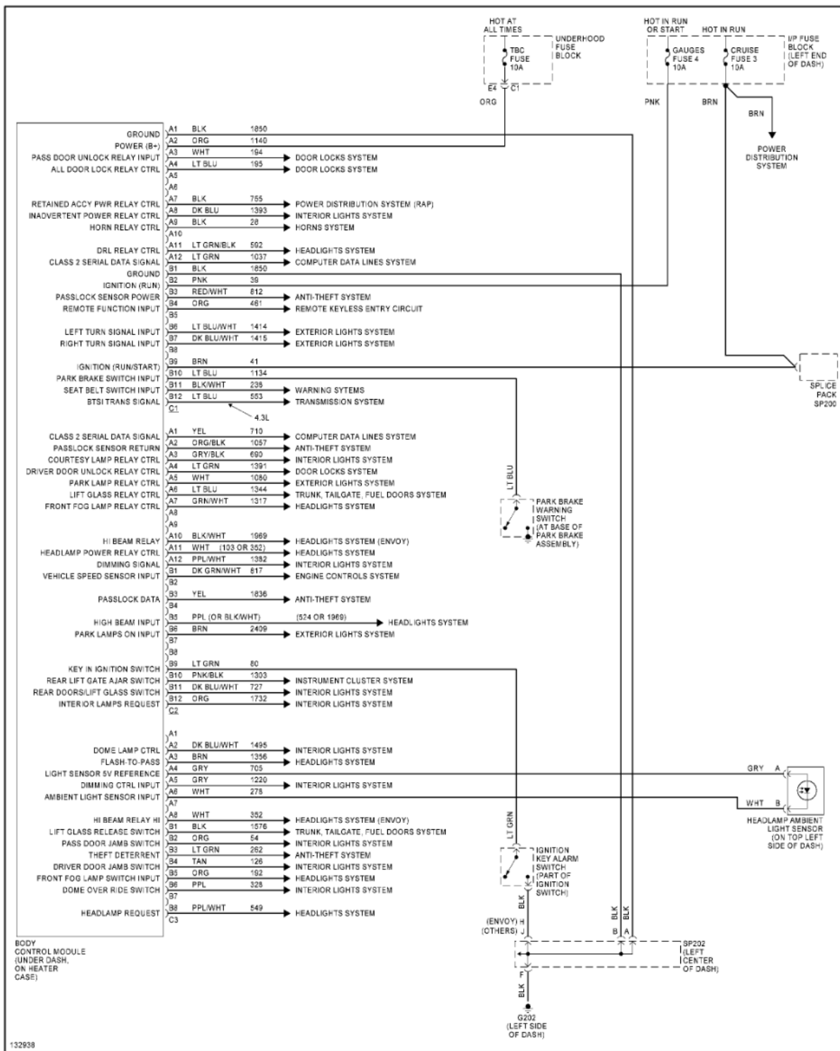
Fig. 13: Body Computer Circuits
