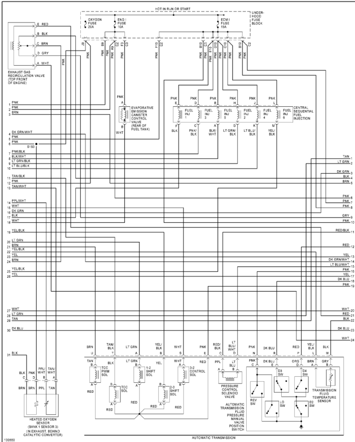
Fig. 24: 4.3L VIN W, Engine Performance Circuits (2 of 4)
