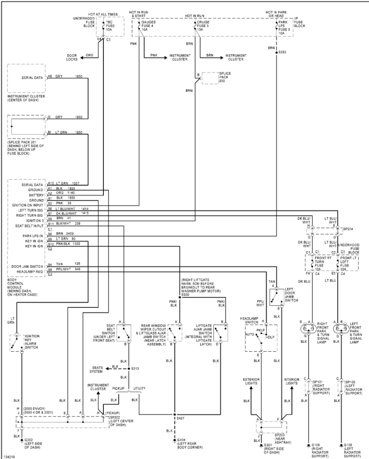
Fig. 63: Warning System Circuits
