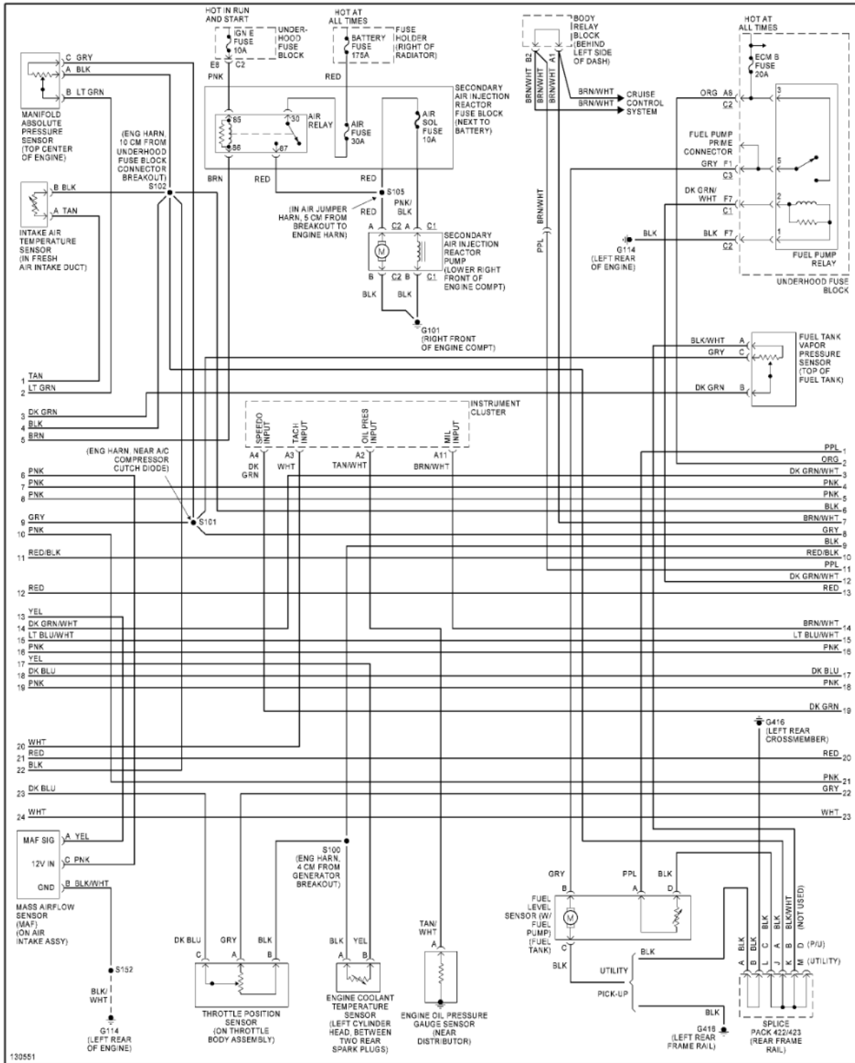
Fig. 25: 4.3L VIN W, Engine Performance Circuits (3 of 4)
