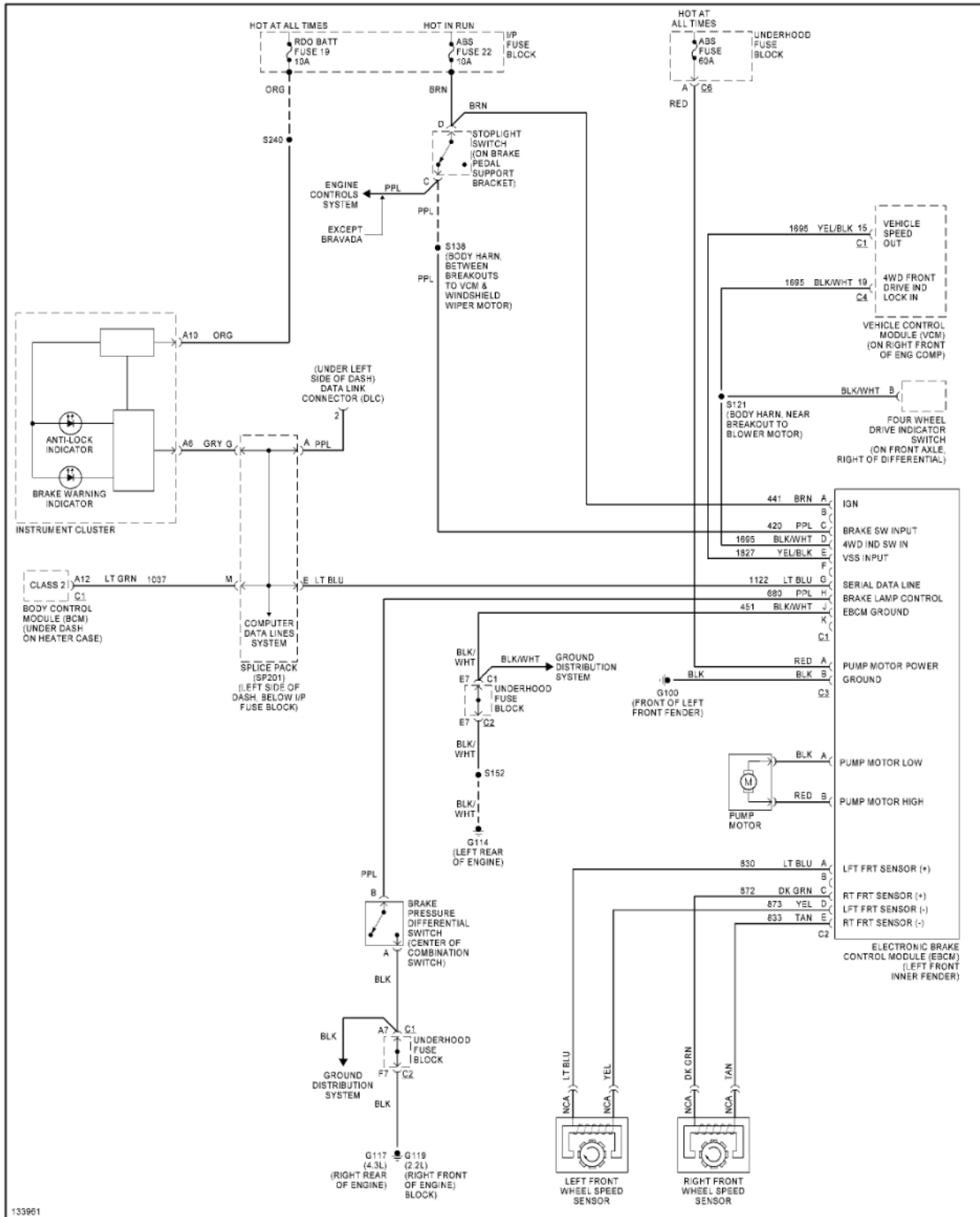
Fig. 9: Anti-lock Brake Circuits, 310 ABS
