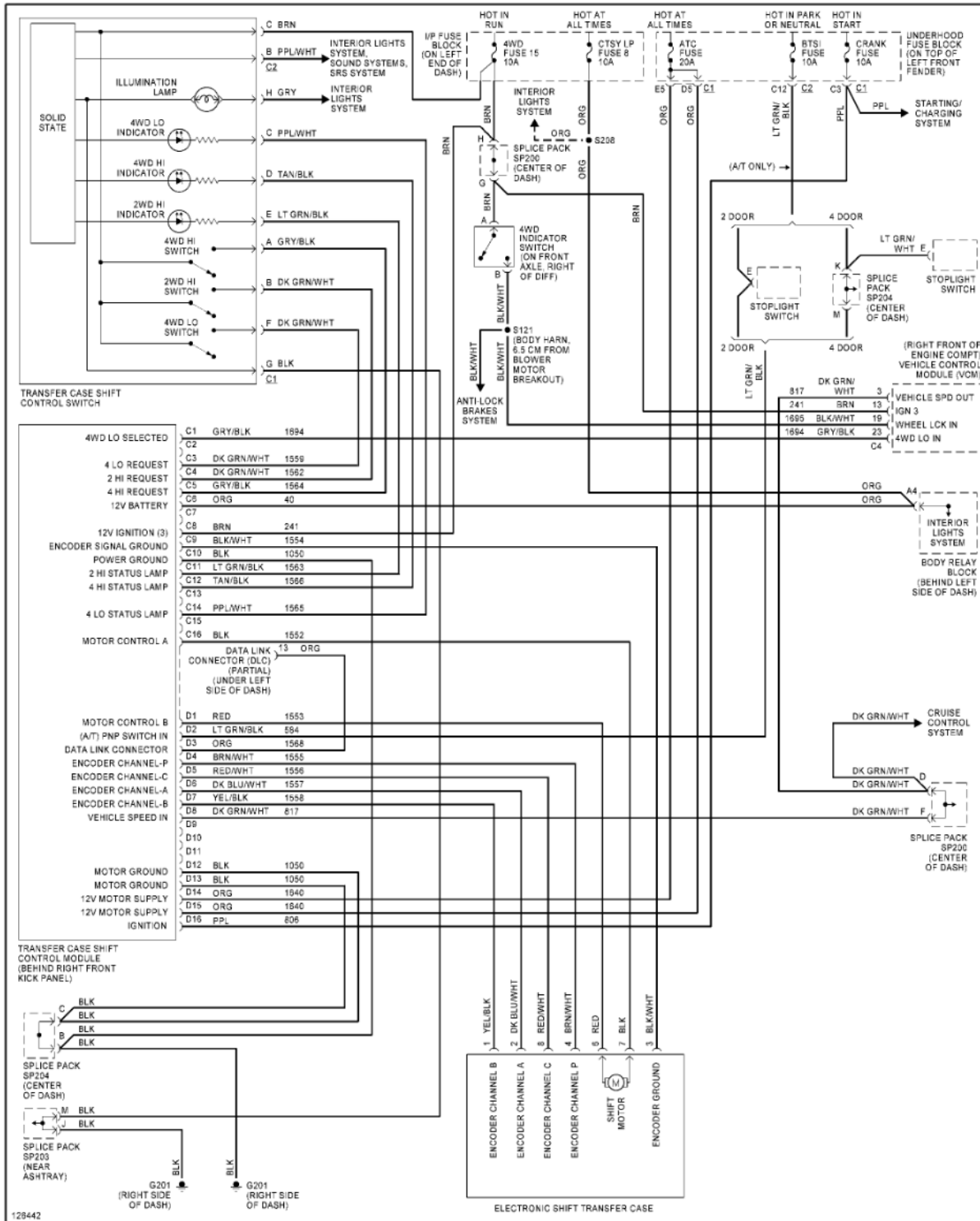
Fig. 62: 4WD Circuit, W/ 2-Speed Selectable Transfer Case
