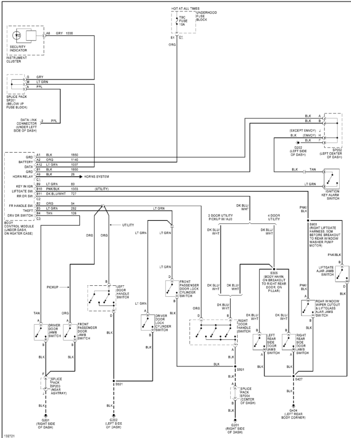
Fig. 11: Forced Entry Circuit
