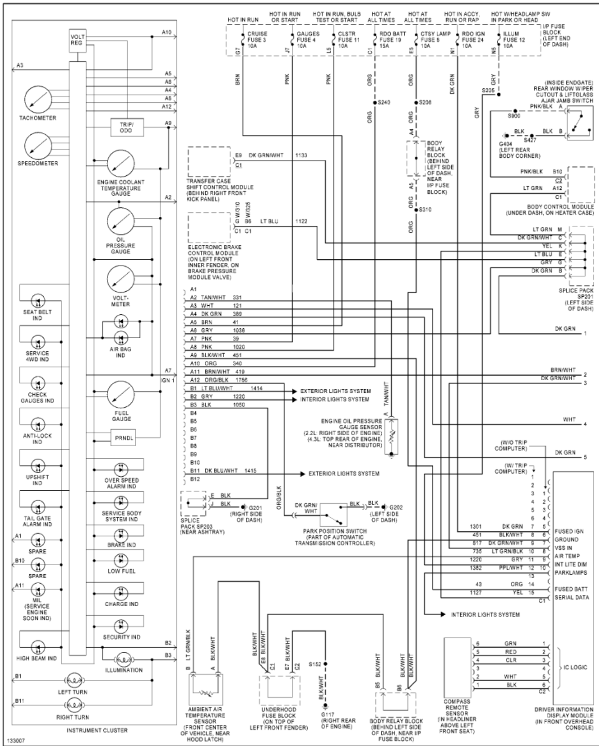
Fig. 35: Instrument Cluster Circuit (1 of 2)
