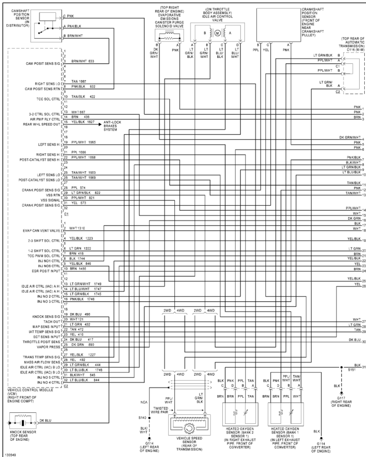
Fig. 23: 4.3L VIN W, Engine Performance Circuits (1 of 4)
