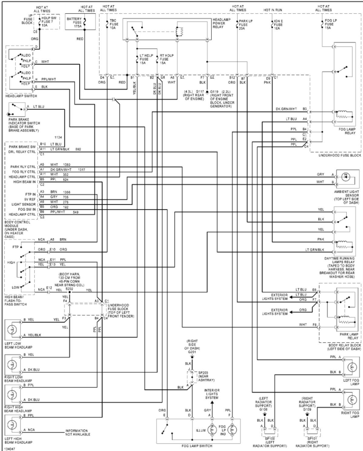
Fig. 32: Headlight Circuit, W/ ZR2
