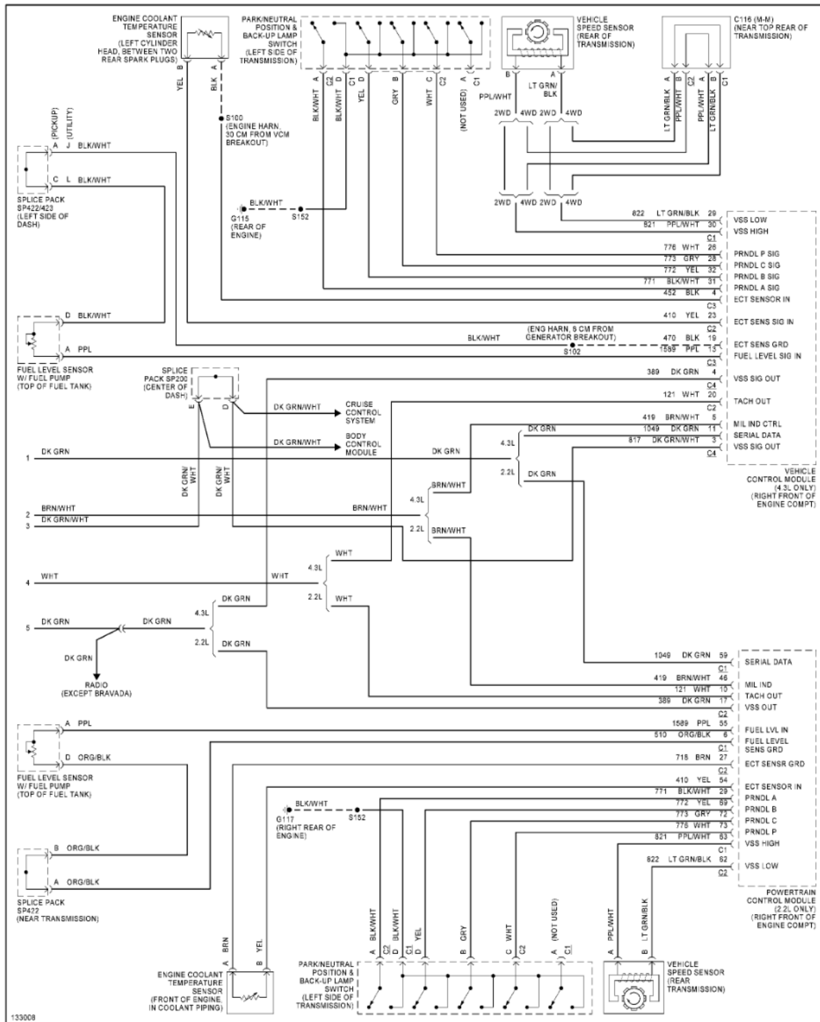
Fig. 36: Instrument Cluster Circuit (2 of 2)
