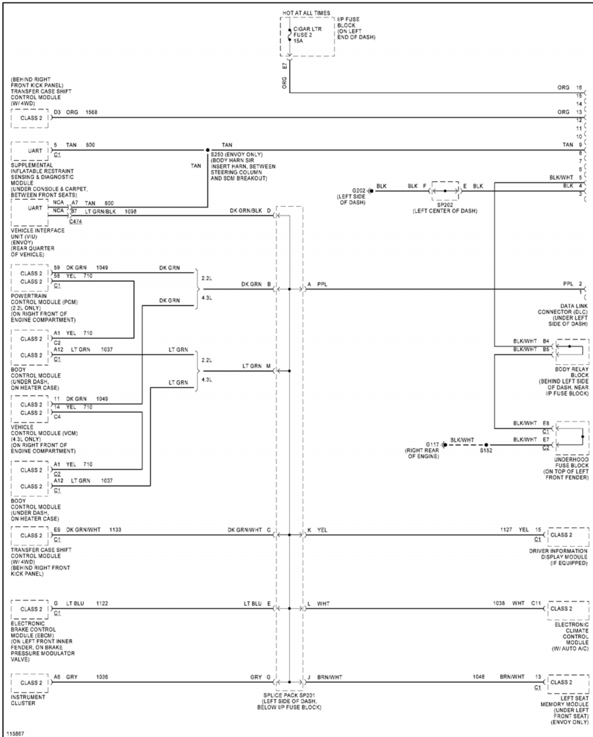
Fig. 13: Computer Data Lines
