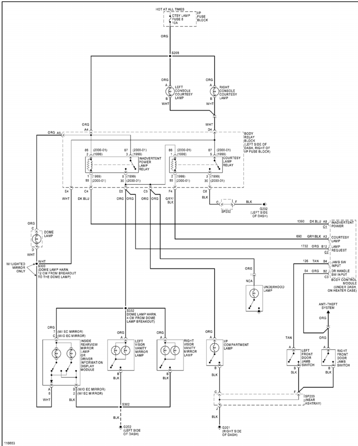
Fig. 36: Courtesy Lamps Circuit
