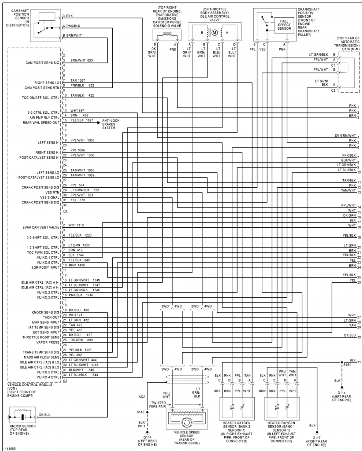
Fig. 19: 4.3L VIN W, Engine Performance Circuits (1 of 4)
