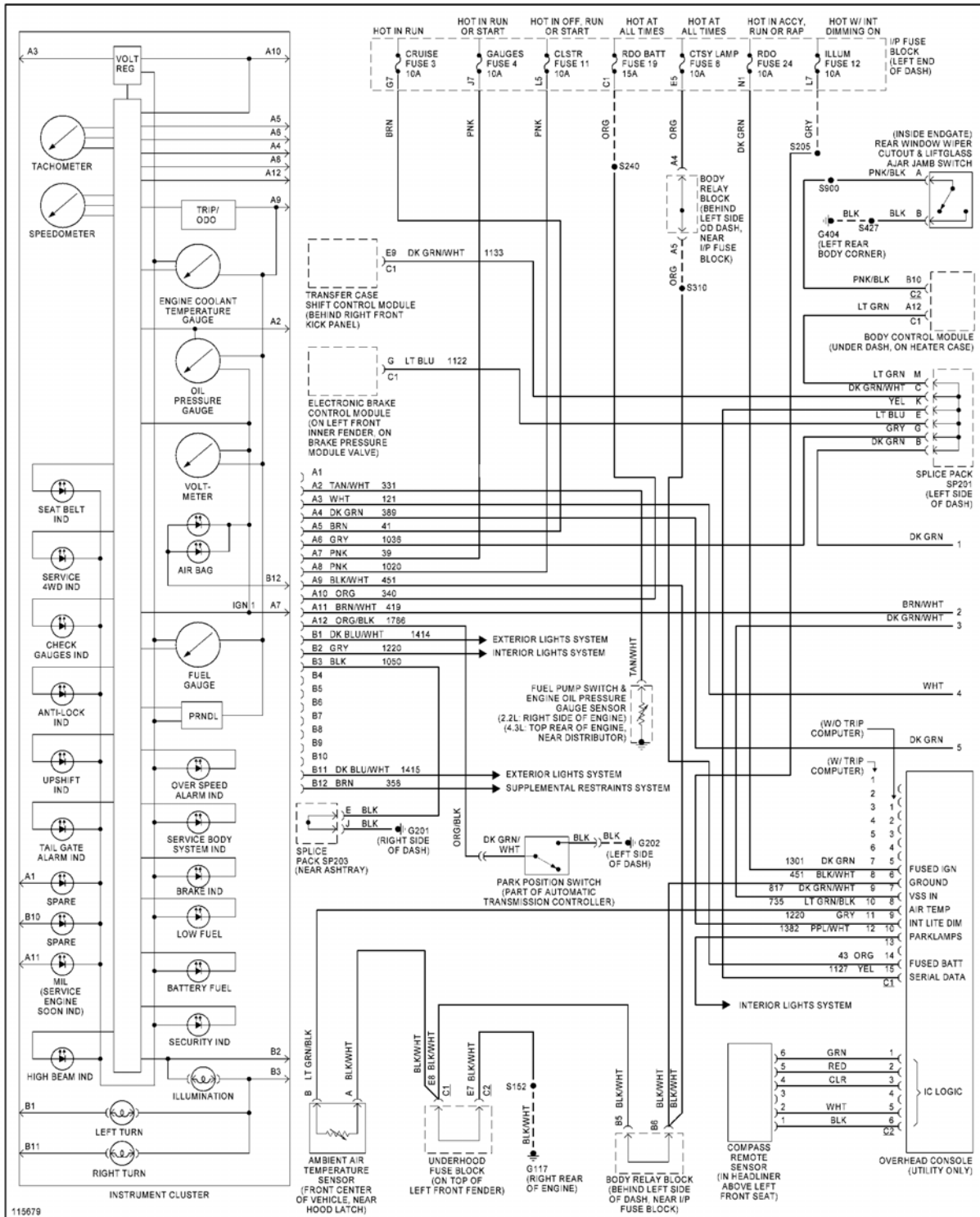
Fig. 34: Instrument Cluster Circuit (1 of 2)
