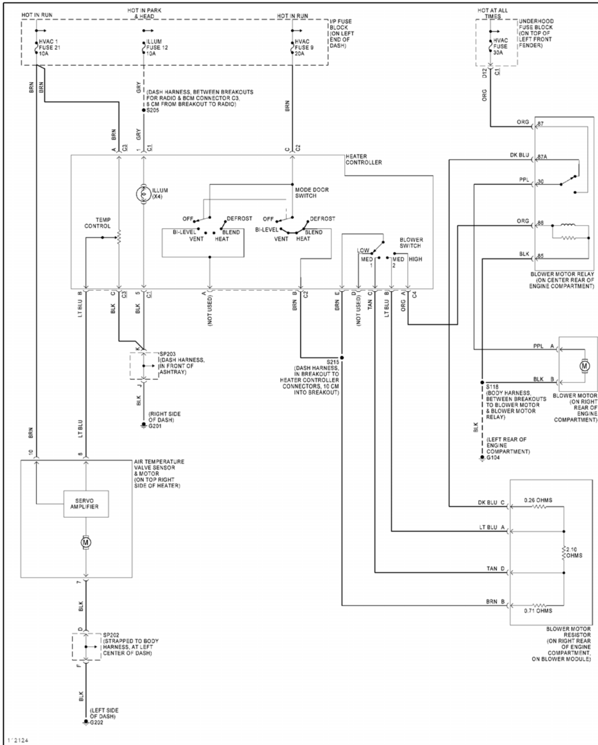
Fig. 8: Heater Circuit
