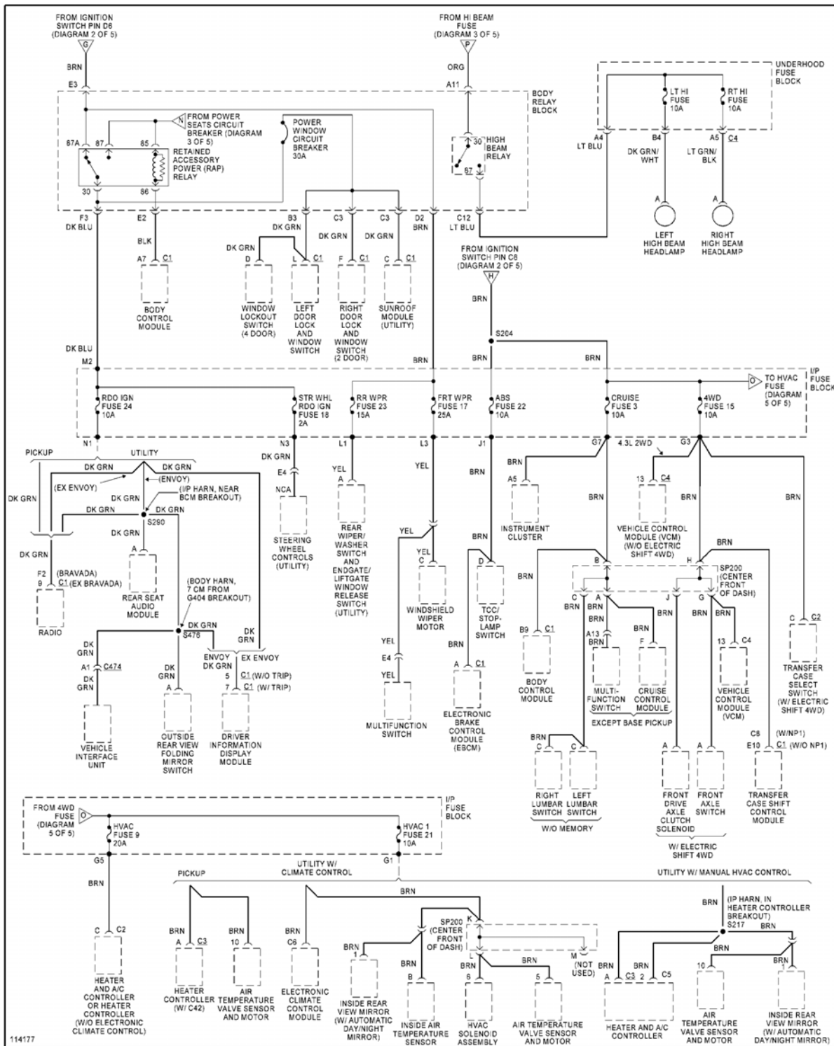
Fig. 42: Power Distribution Circuit (5 of 5)
