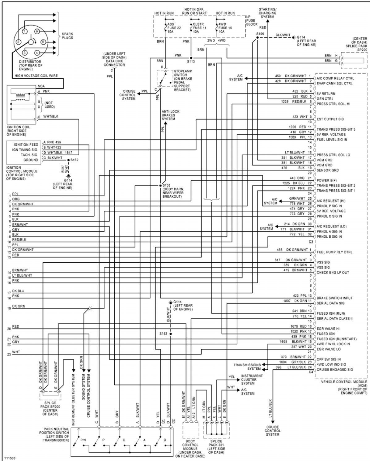
Fig. 22: 4.3L VIN W, Engine Performance Circuits (4 of 4)
