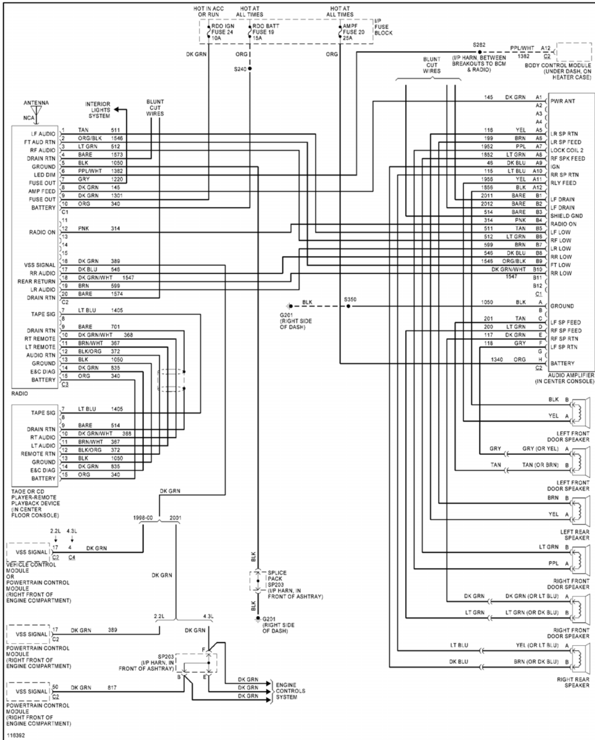
Fig. 47: Radio Circuits, W/ Amplifier
