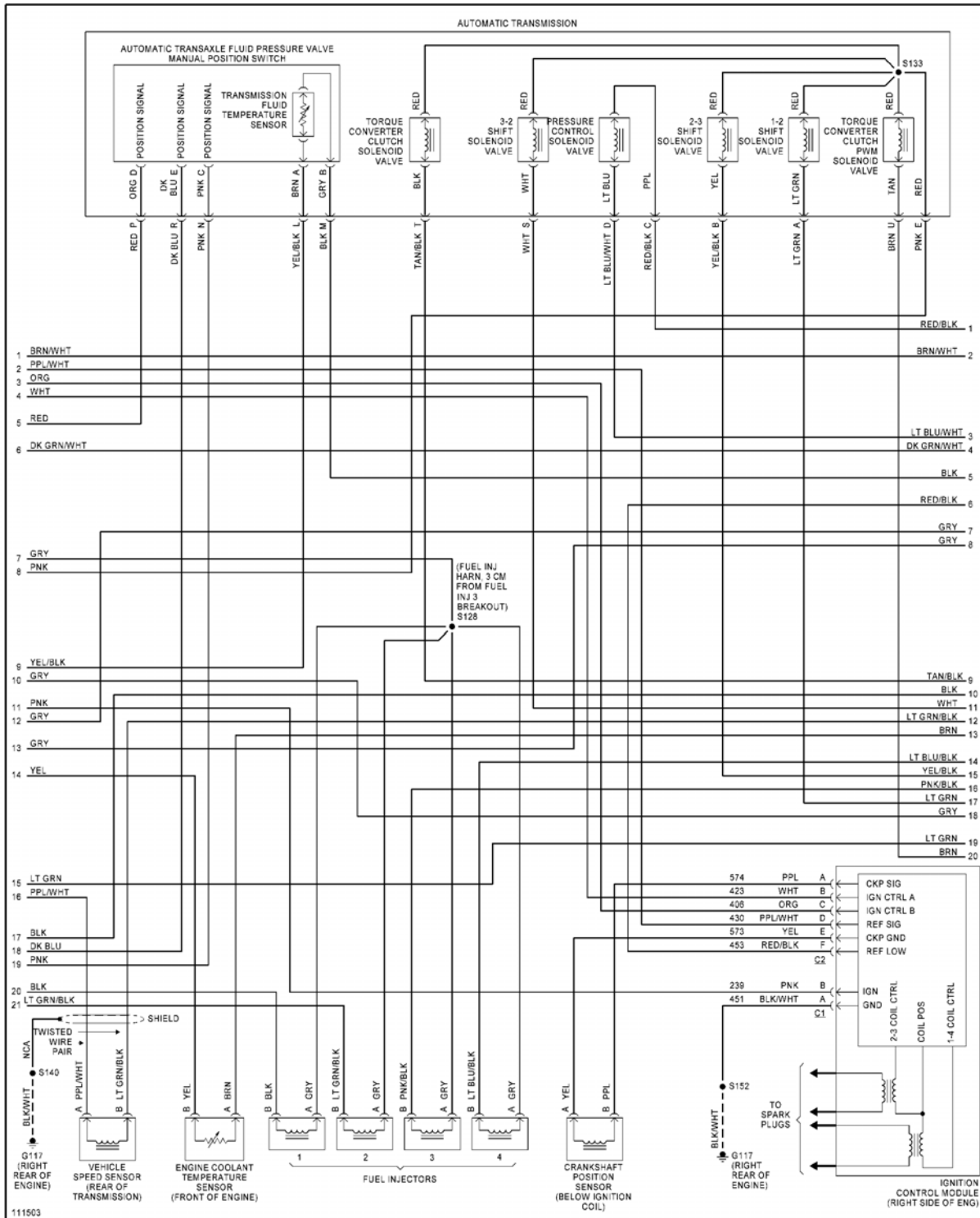
Fig. 17: 2.2L VIN 4, Engine Performance Circuits (2 of 3)
