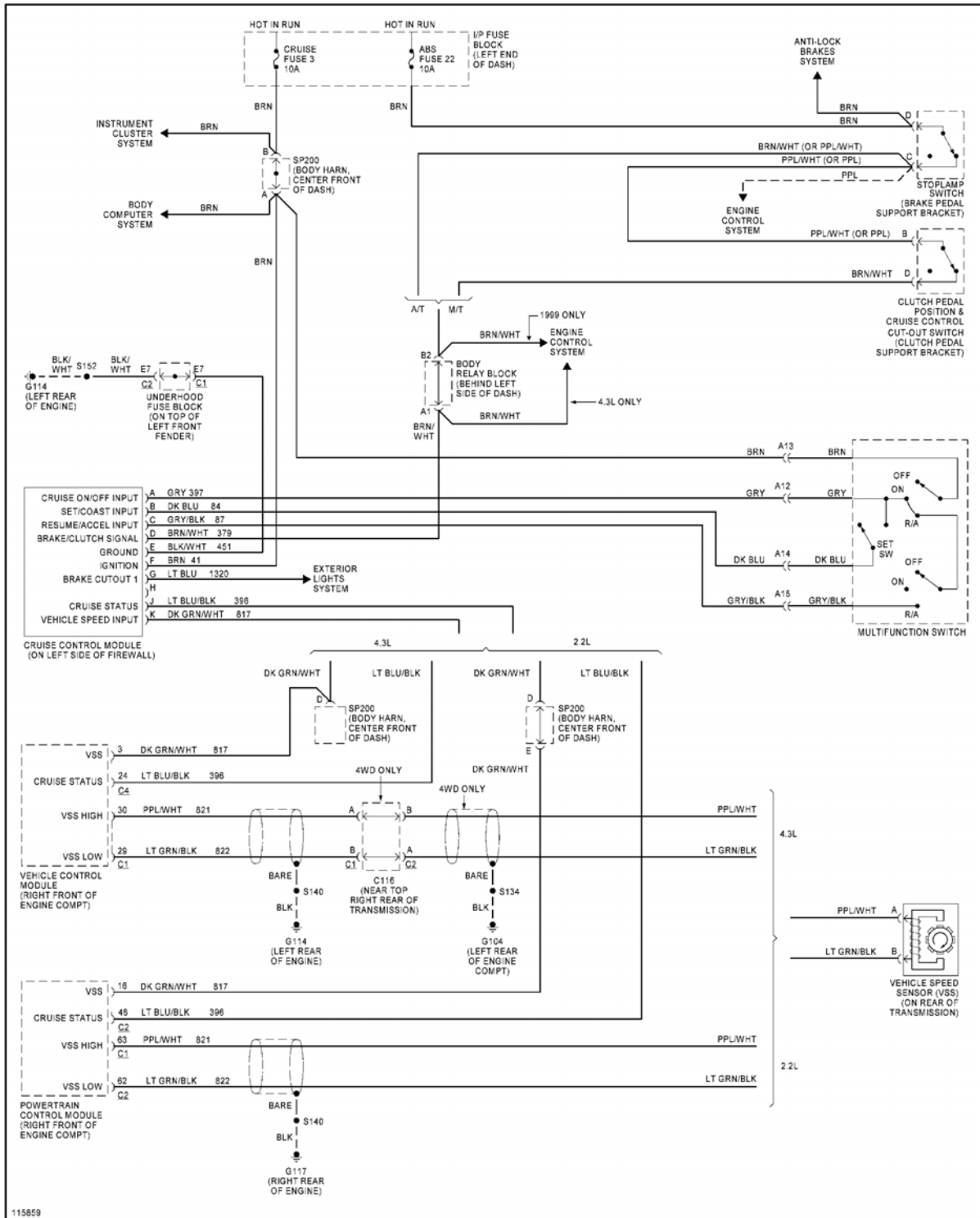
Fig. 14: Cruise Control Circuit
