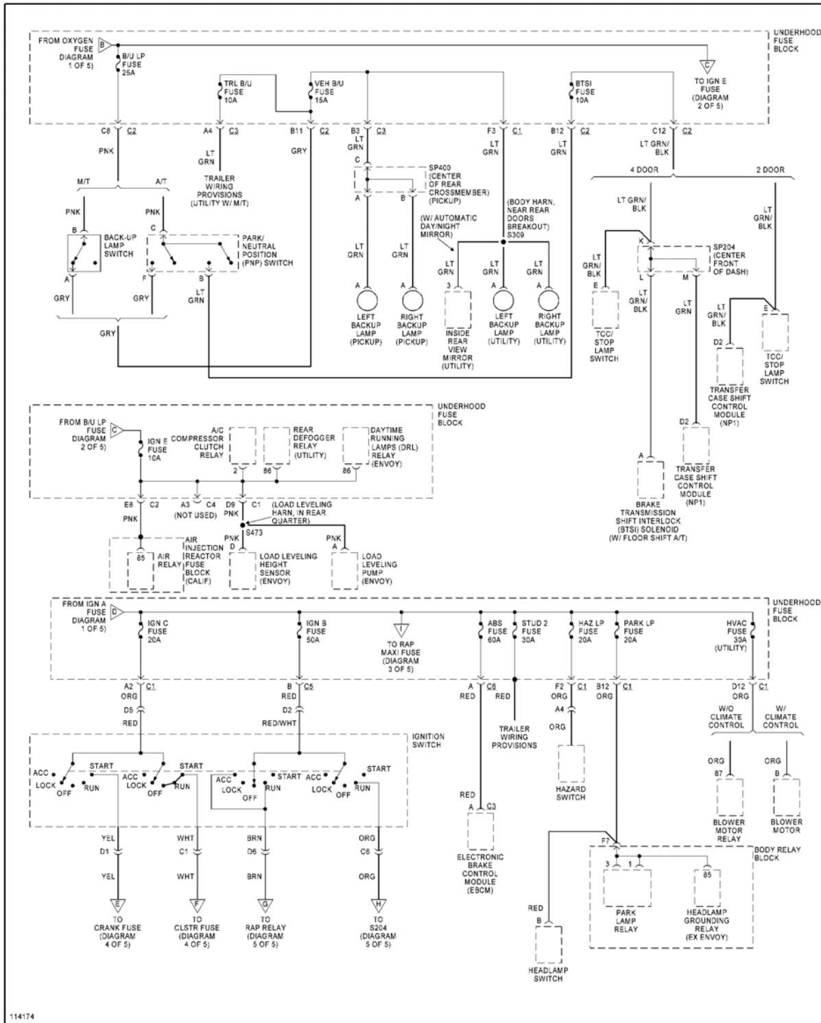
Fig. 39: Power Distribution Circuit (2 of 5)
