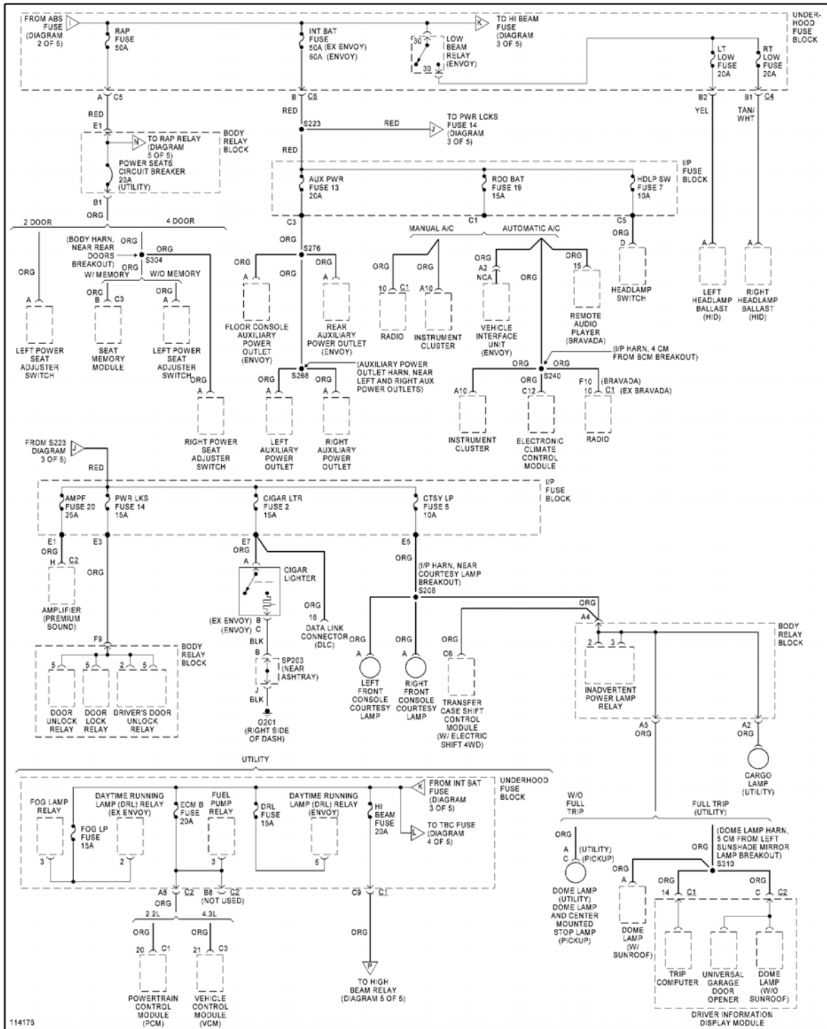
Fig. 40: Power Distribution Circuit (3 of 5)
