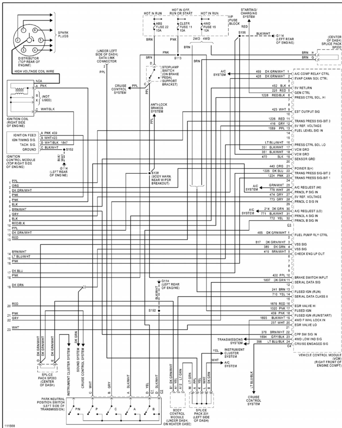
Fig. 26: 4.3L VIN X, Engine Performance Circuits (4 of 4)
