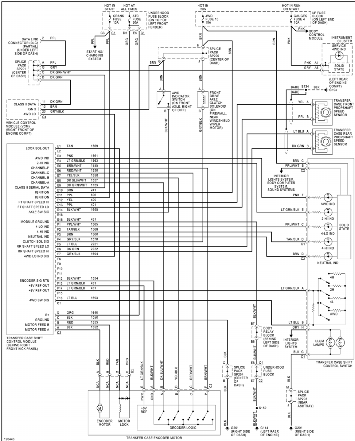
Fig. 54: 4WD Circuit, W/ 2-Speed Automatic Transfer Case
