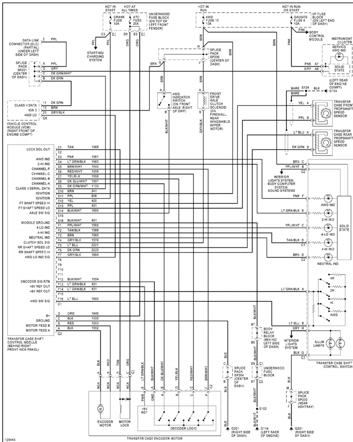
Fig. 58: 4WD Circuit, W/ 2-Speed Automatic Transfer Case
