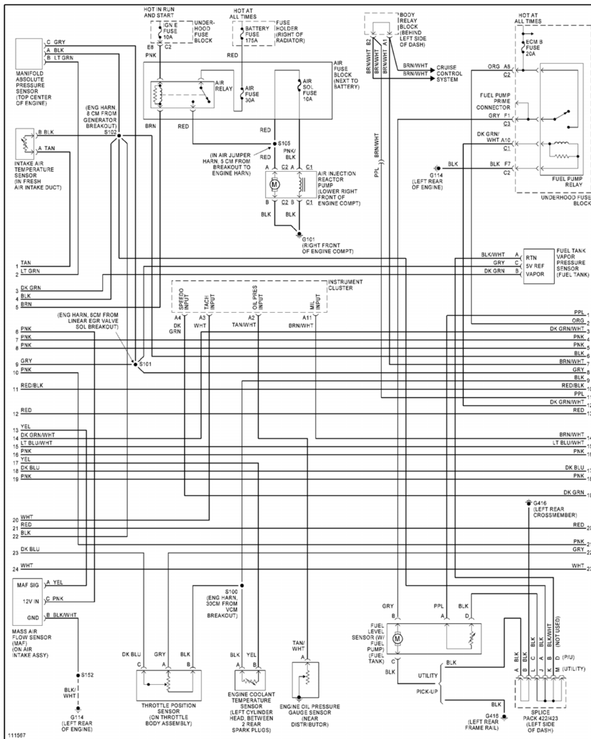
Fig. 25: 4.3L VIN X, Engine Performance Circuits (3 of 4)
