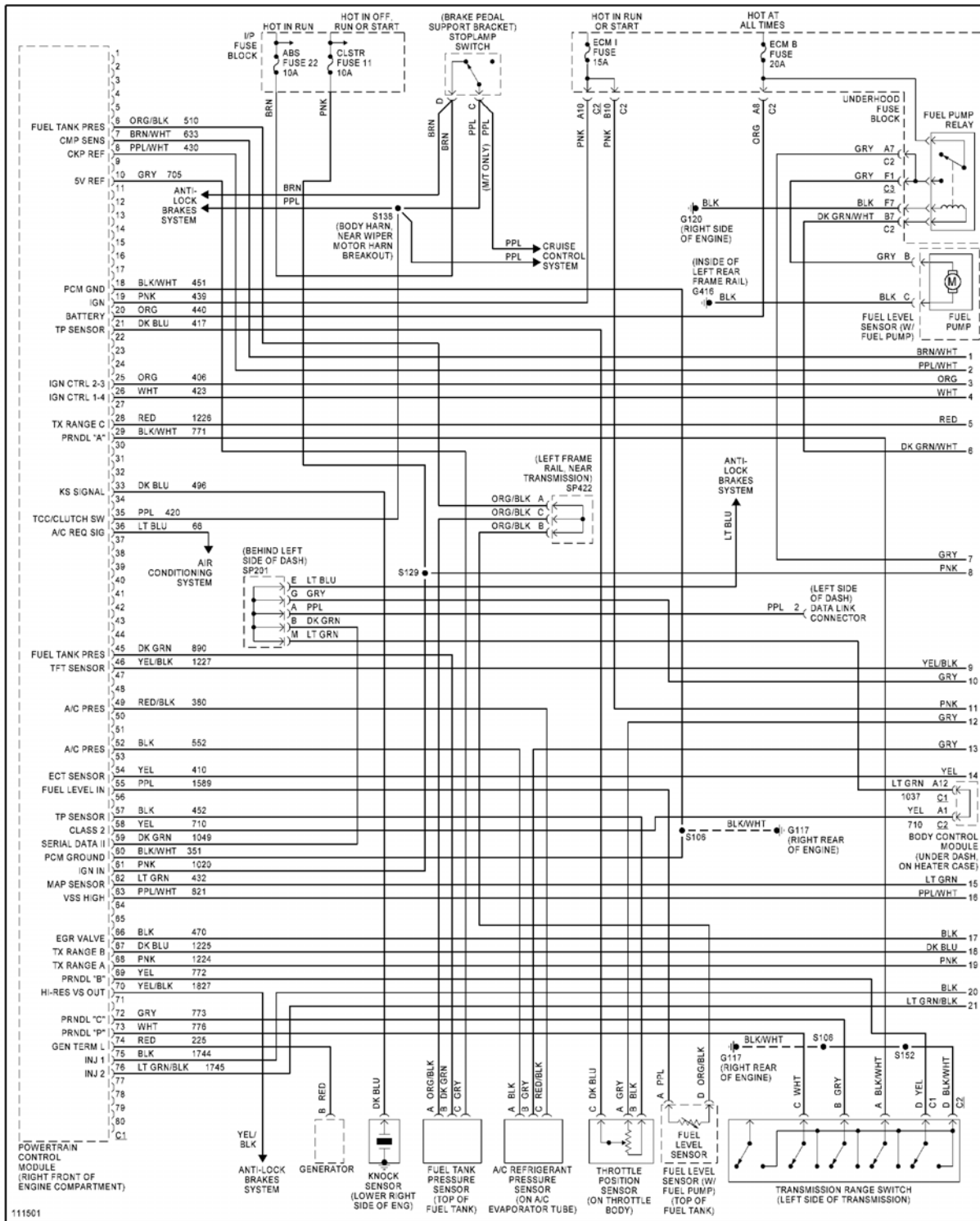
Fig. 16: 2.2L VIN 4, Engine Performance Circuits (1 of 3)
