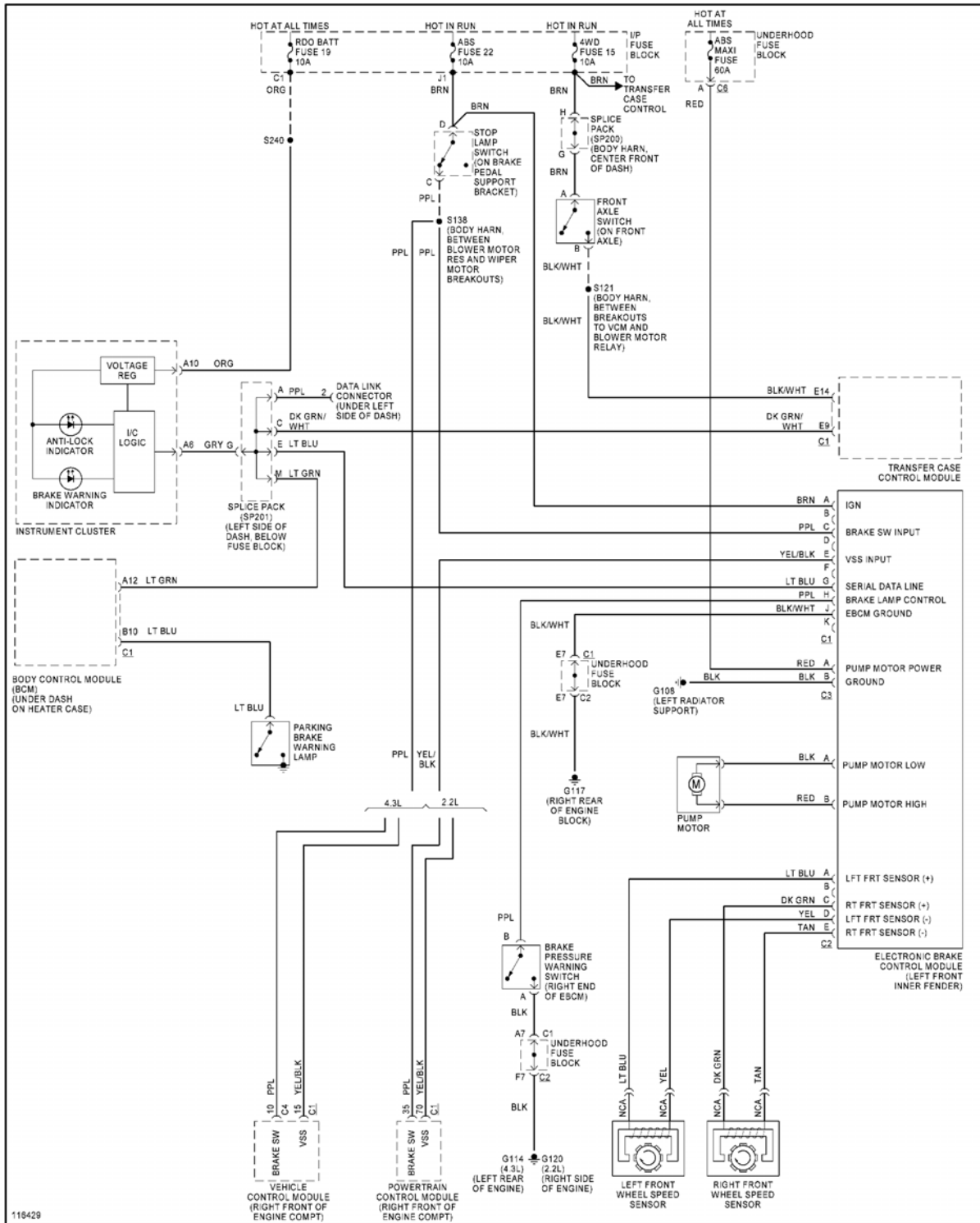
Fig. 9: Anti-lock Brake Circuits
