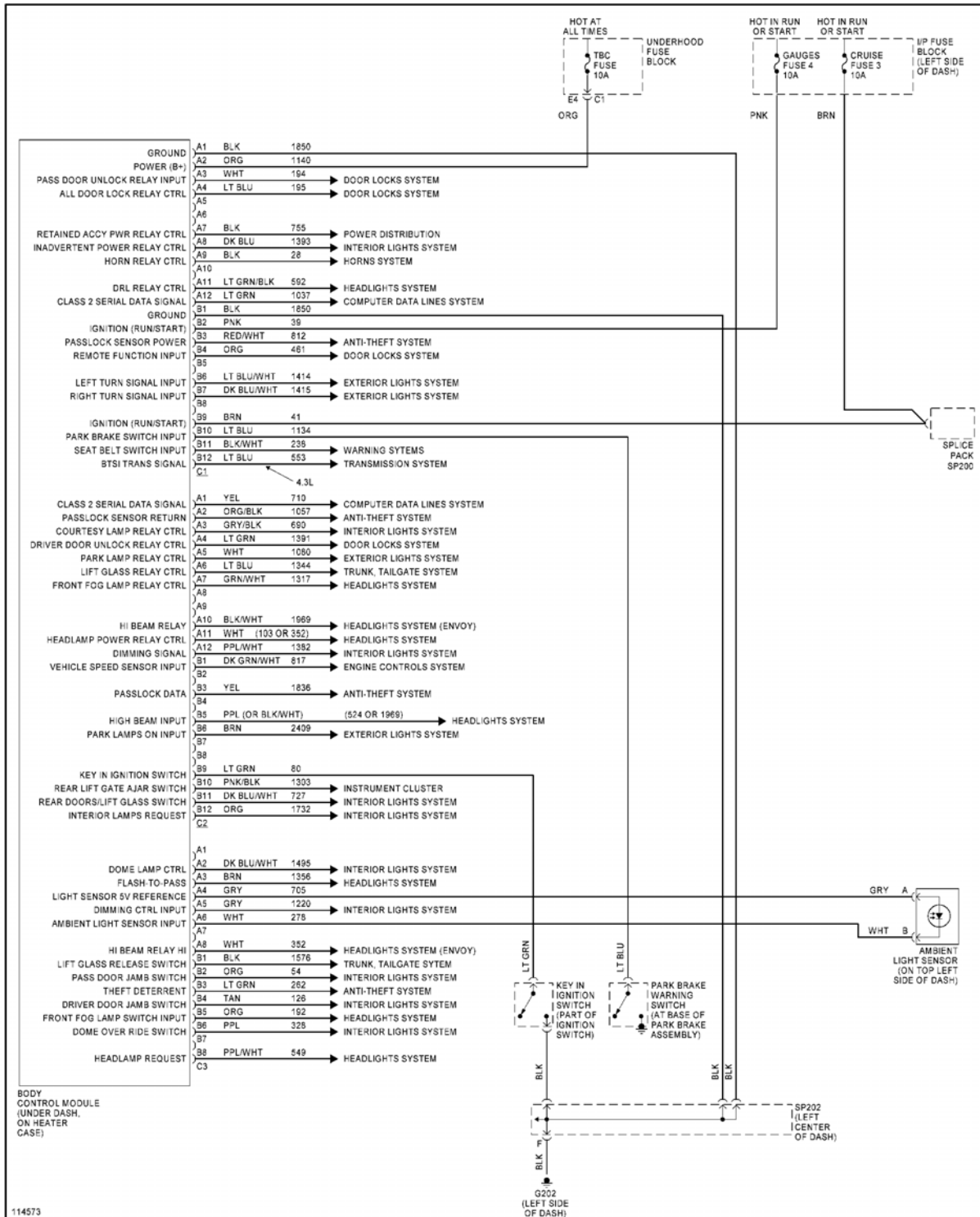
Fig. 12: Body Computer Circuits
