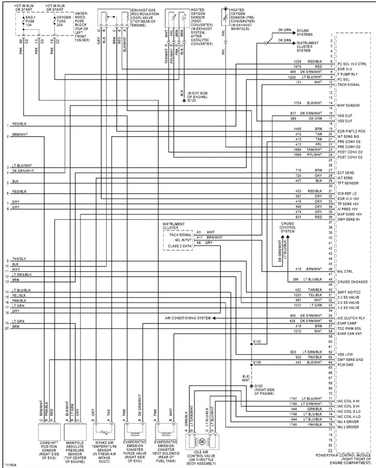
Fig. 18: 2.2L VIN 4, Engine Performance Circuits (3 of 3)
