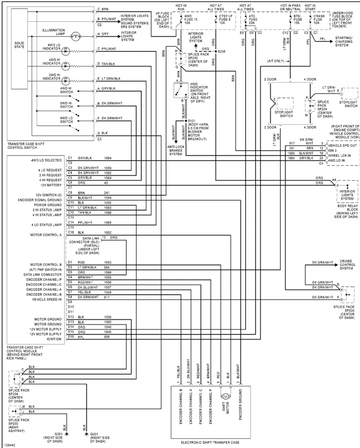
Fig. 59: 4WD Circuit, W/ 2-Speed Selectable Transfer Case
