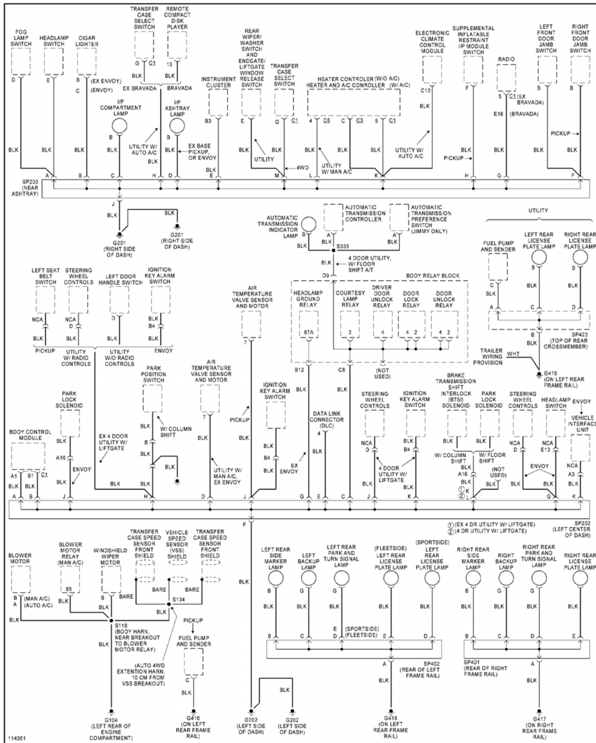
Fig. 30: Ground Distribution Circuit (2 of 3)
