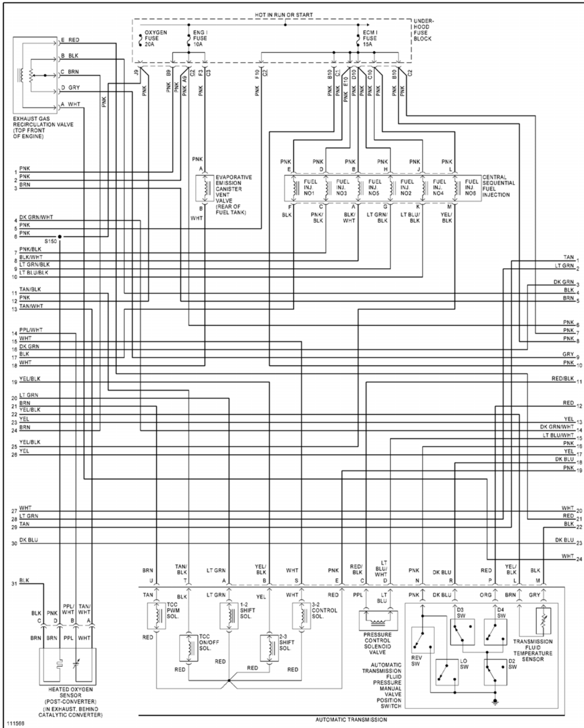
Fig. 20: 4.3L VIN W, Engine Performance Circuits (2 of 4)
