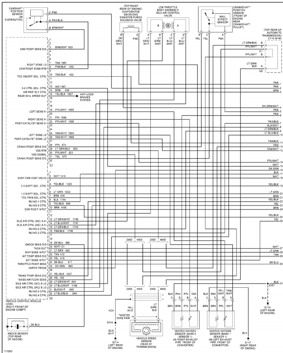
Fig. 23: 4.3L VIN X, Engine Performance Circuits (1 of 4)
