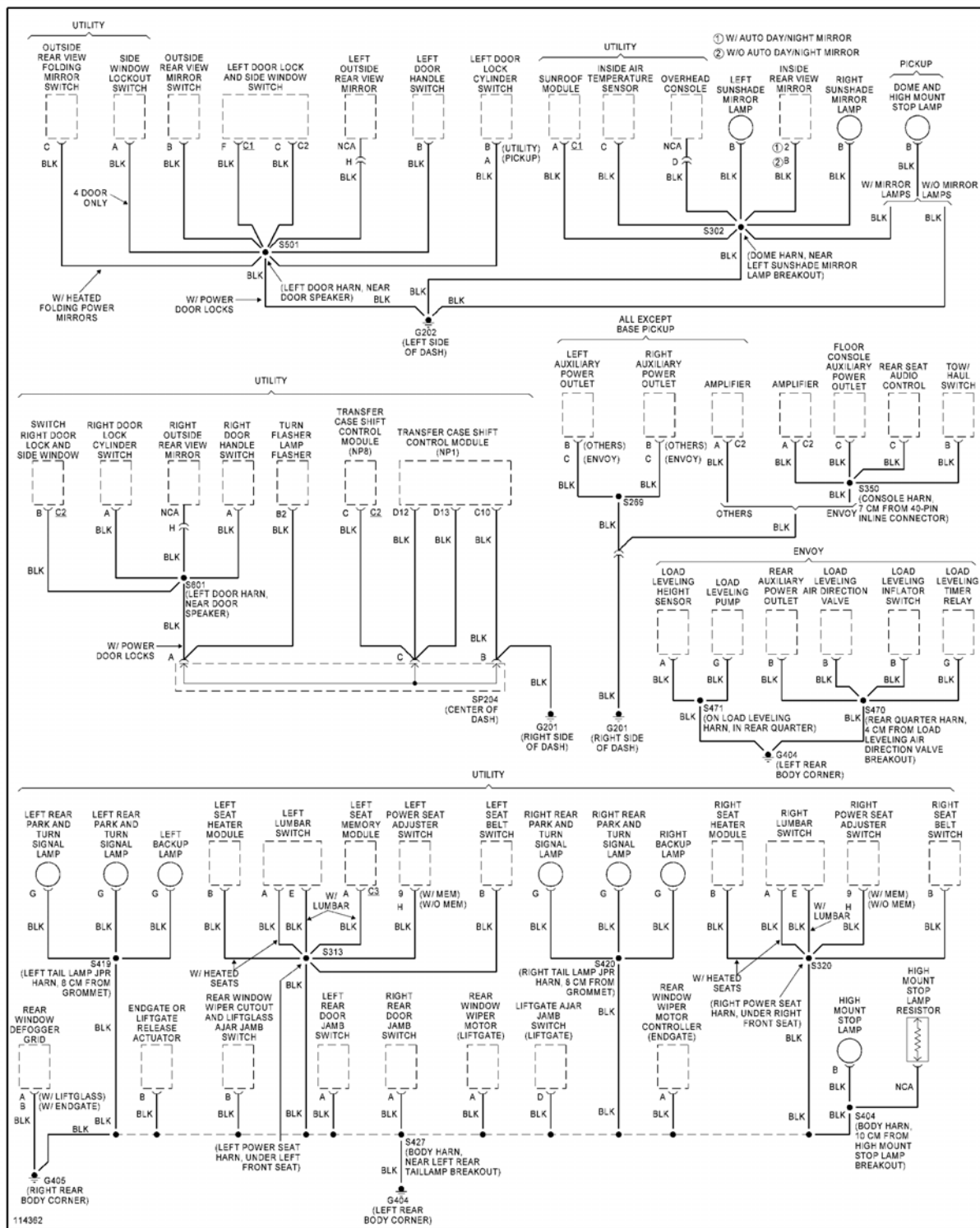
Fig. 31: Ground Distribution Circuit (3 of 3)
