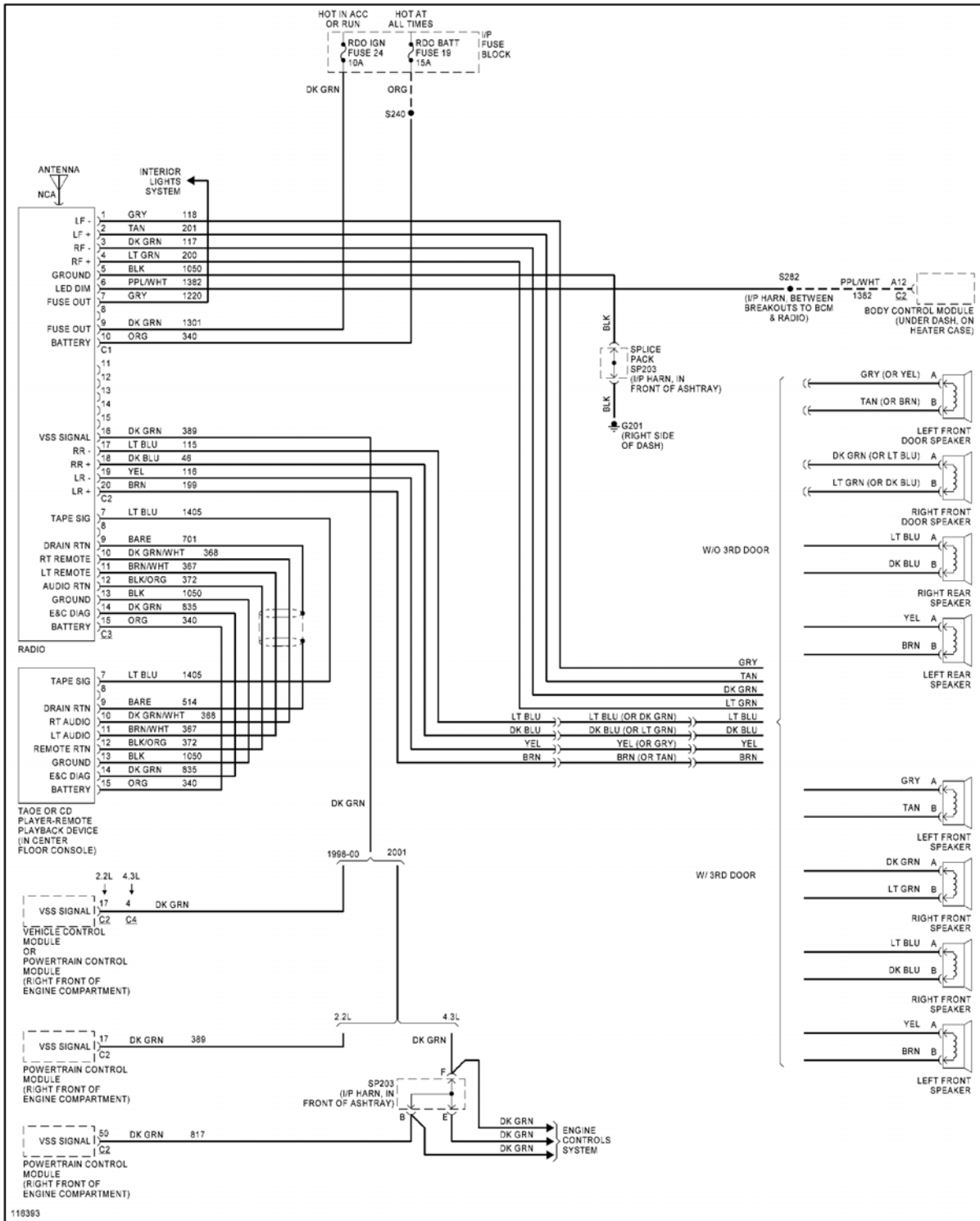
Fig. 48: Radio Circuits, W/O Amplifier
