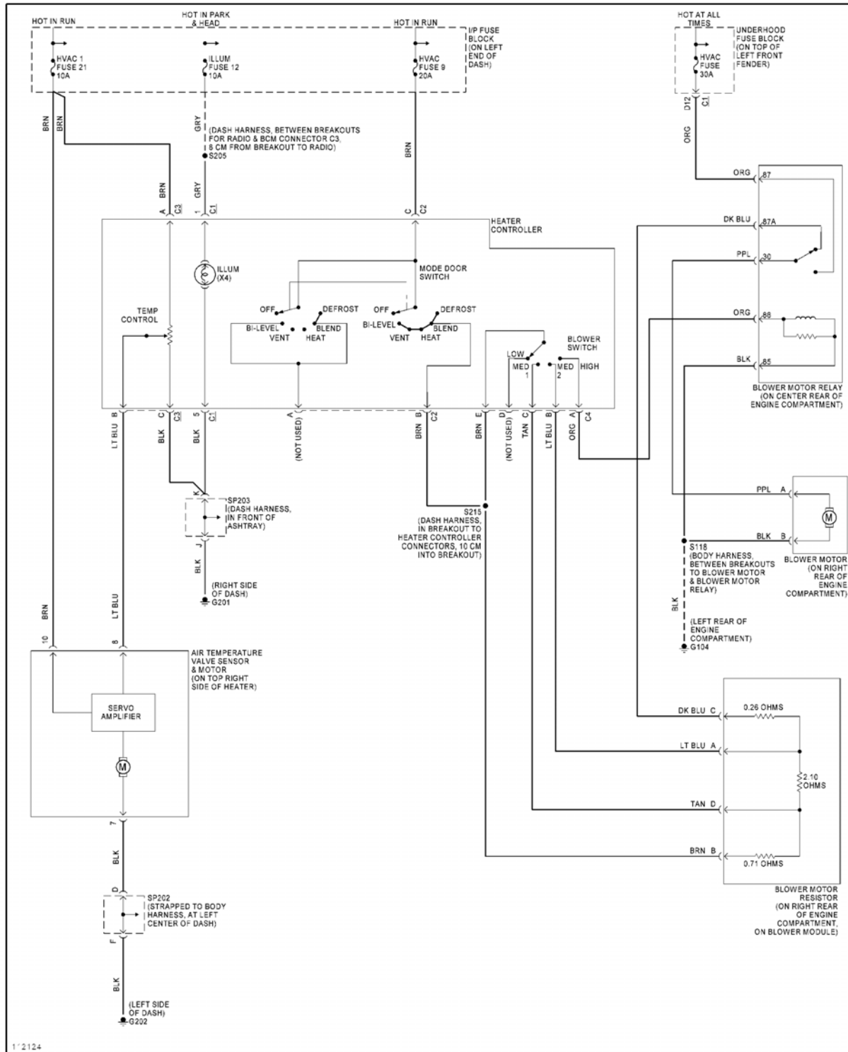
Fig. 3: Heater Circuit
