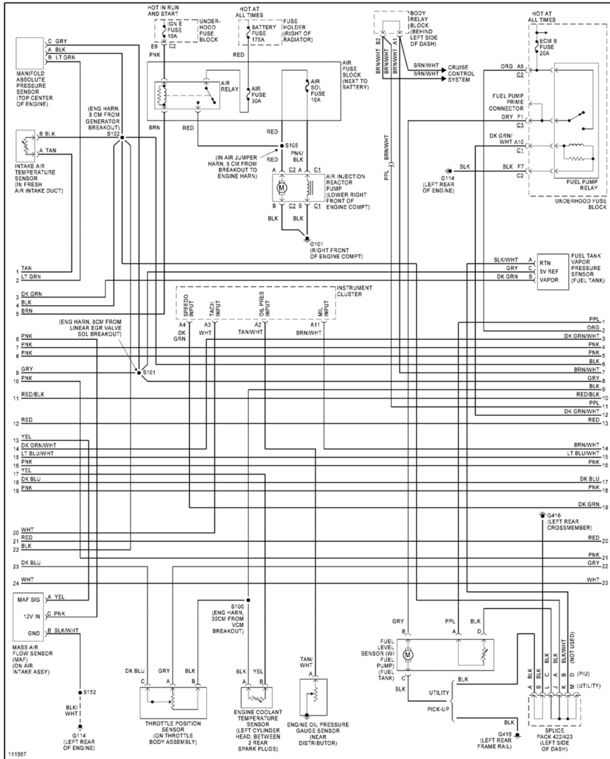
Fig. 21: 4.3L VIN W, Engine Performance Circuits (3 of 4)
