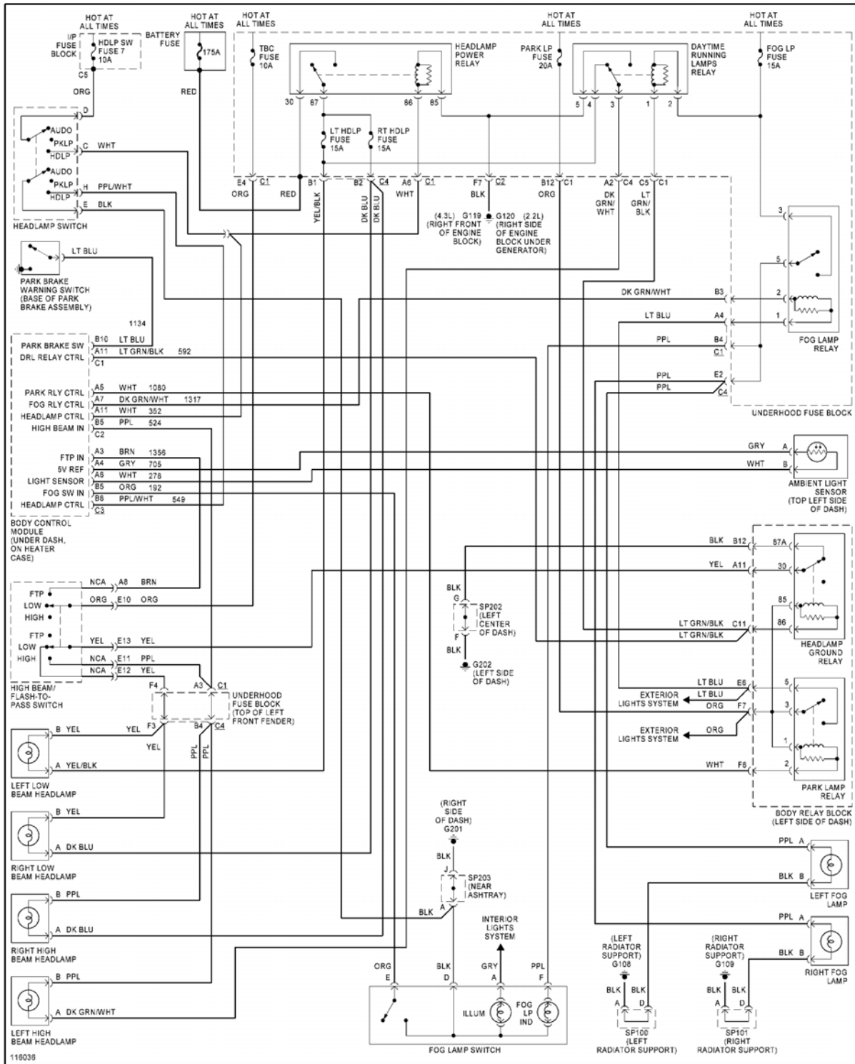
Fig. 32: Headlight Circuit
