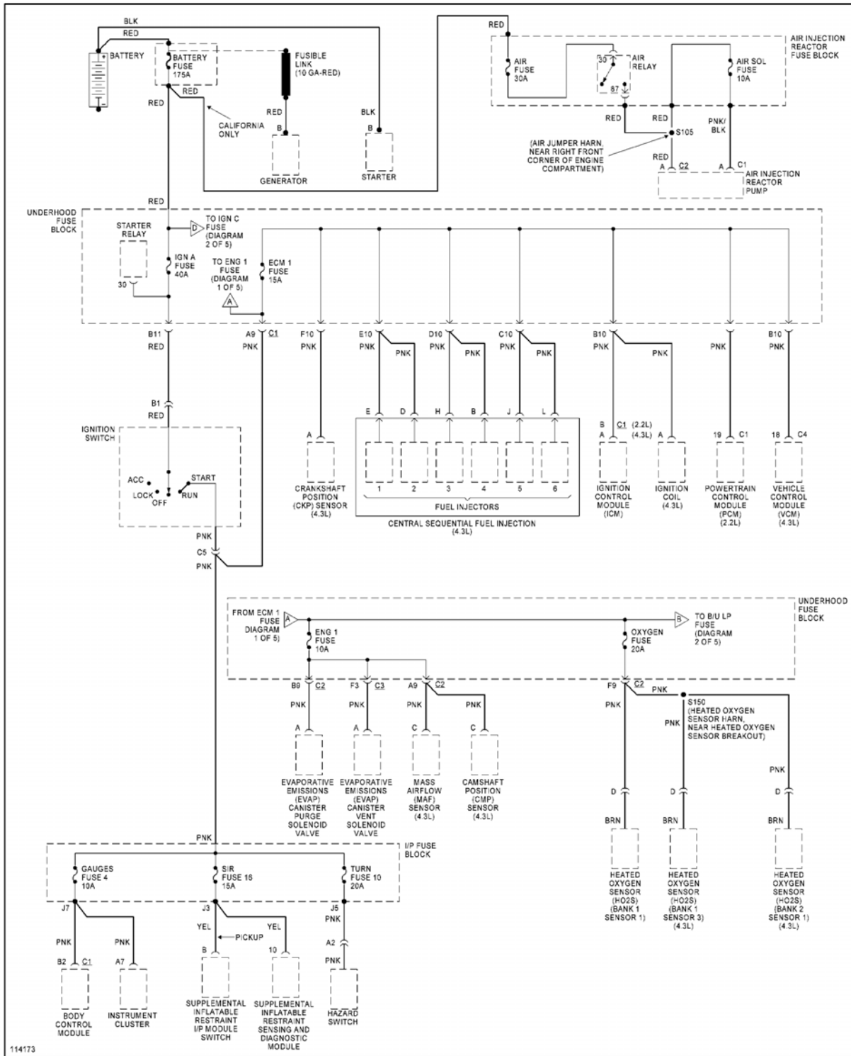
Fig. 38: Power Distribution Circuit (1 of 5)
