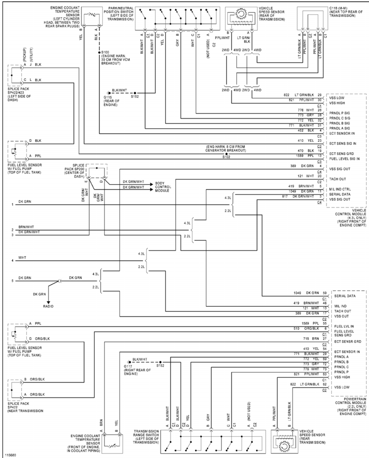
Fig. 35: Instrument Cluster Circuit (2 of 2)
