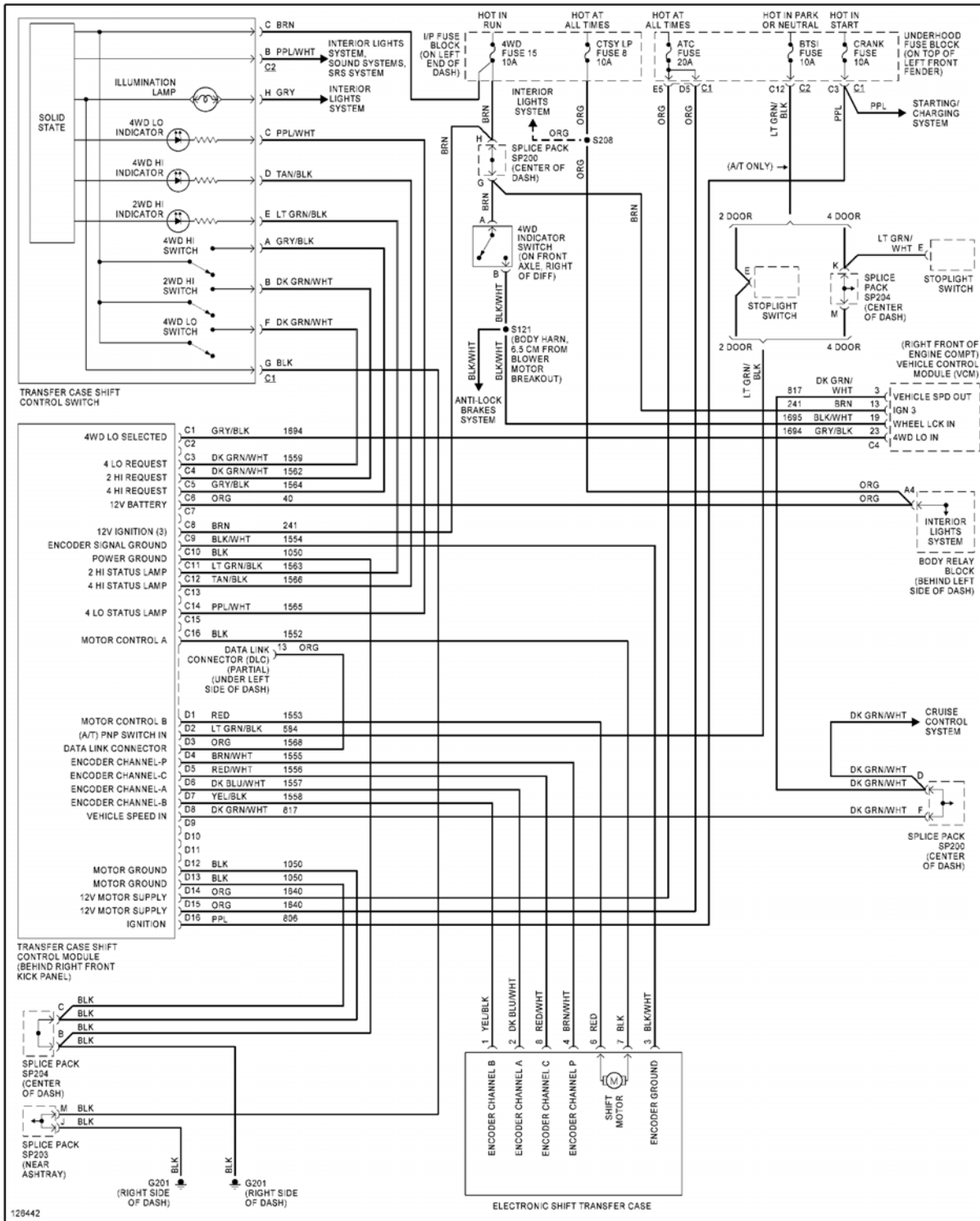
Fig. 55: 4WD Circuit, W/ 2-Speed Selectable Transfer Case
