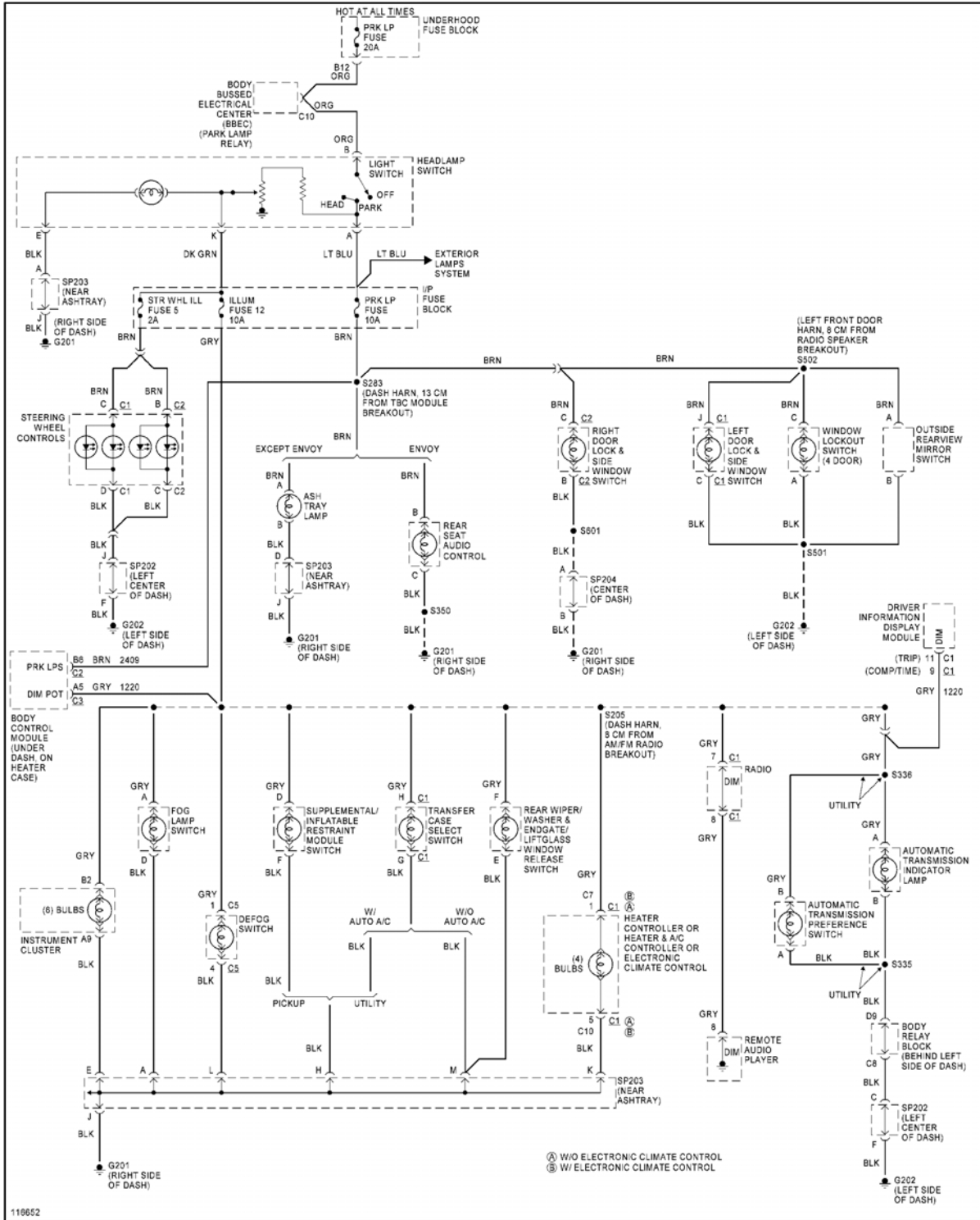
Fig. 37: Instrument Illumination Circuit
