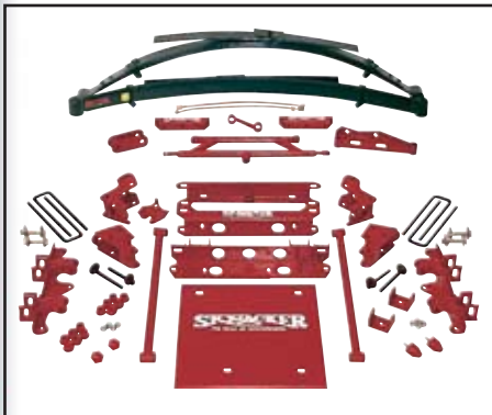
SJ4636B - Lift System 1993-98 pickup
