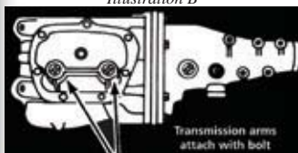
Muncie, G.M., 7 bolt side cover used 1969 & later
