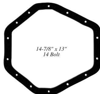
GM-14 Bolt-10.5" Ring Gear
